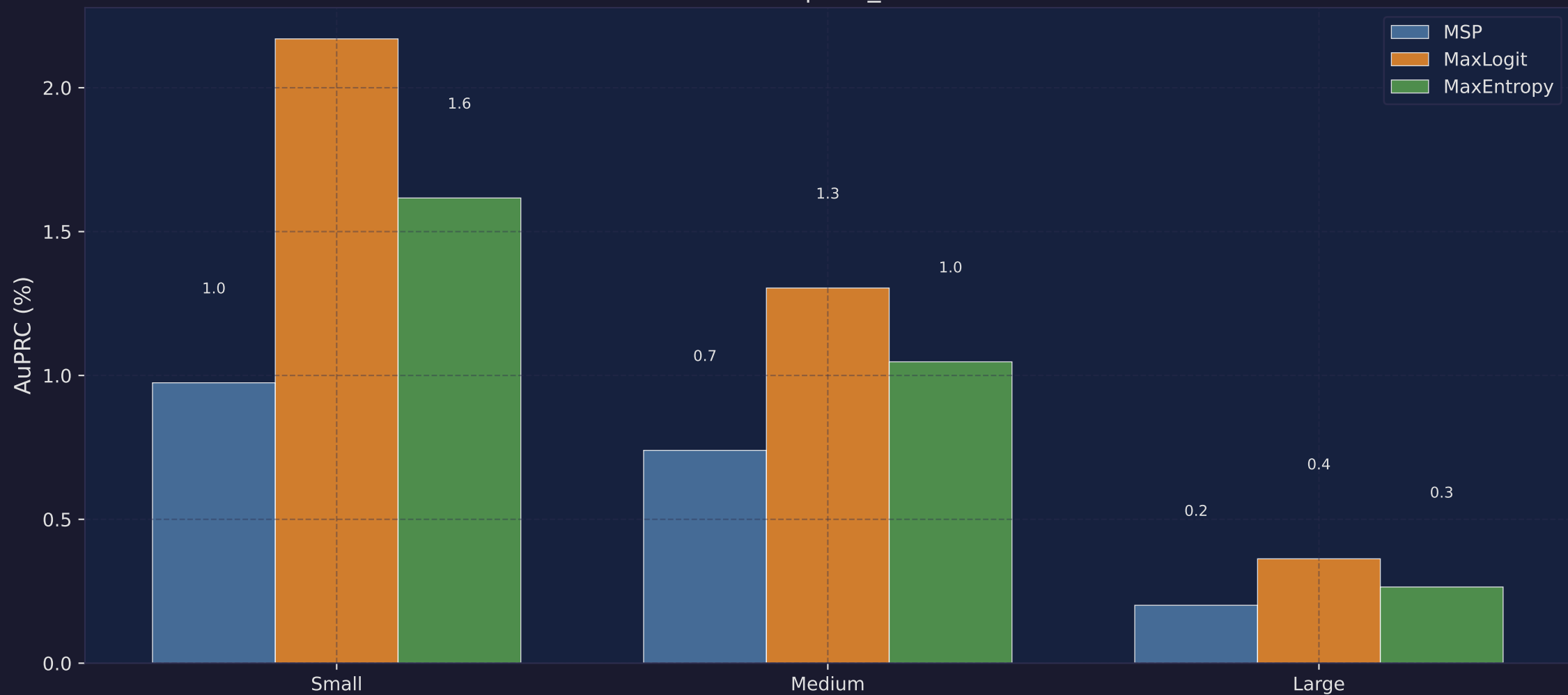
AuPRC by Anomaly Size Bucket ERFNet | lost_found
