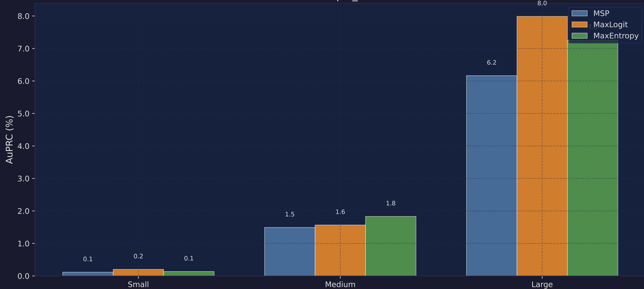
AuPRC by Anomaly Size Bucket ERFNet | fs_static
