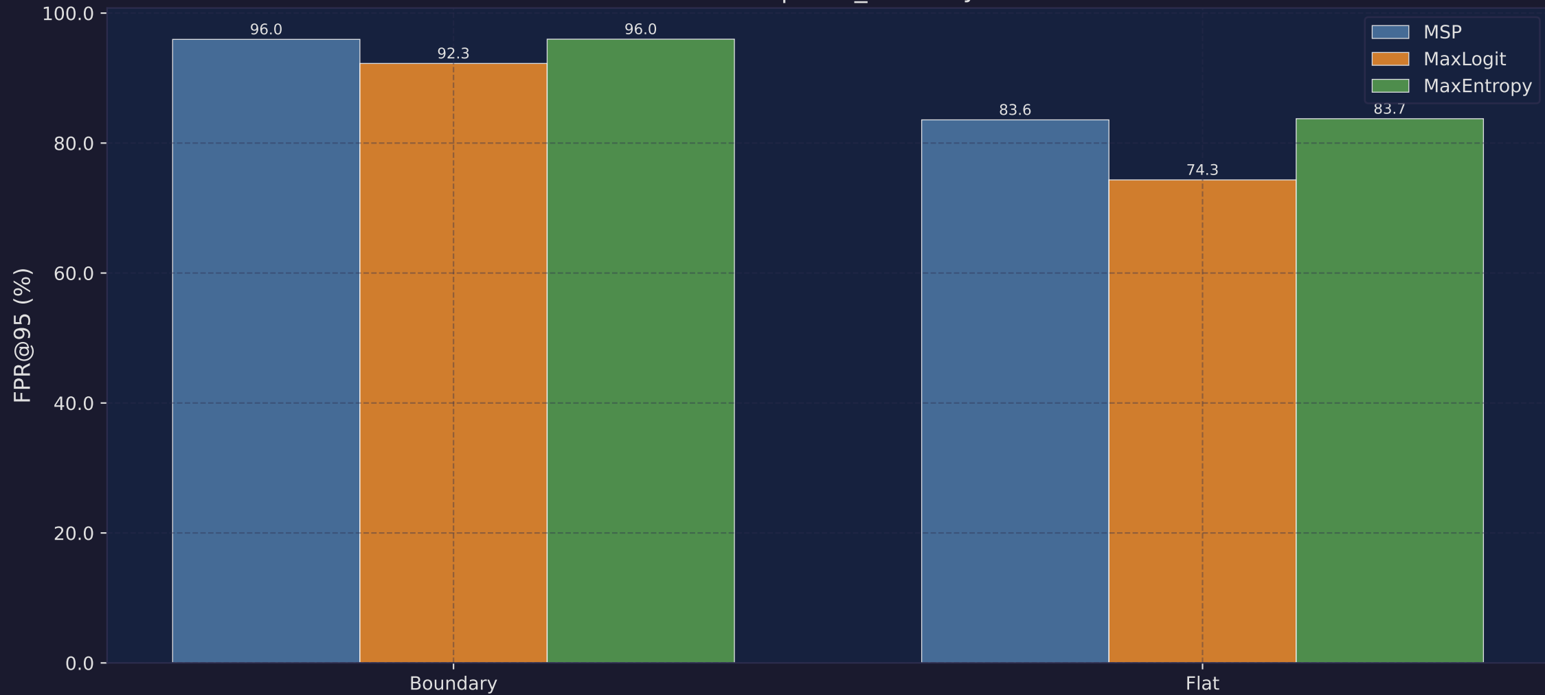
FPR@95 — Boundary vs Flat Region ERFNet | road_anomaly
