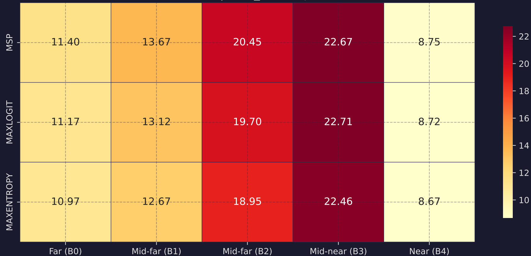
FPR@95 (%) by Depth Band EoMT | road_anomaly
