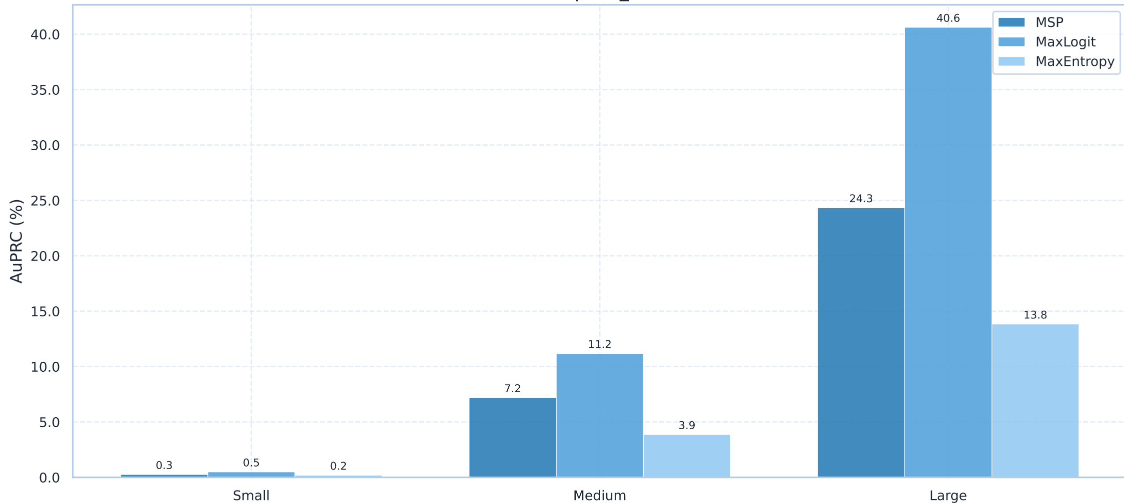
AuPRC by Anomaly Size Bucket EoMT | lost_found
