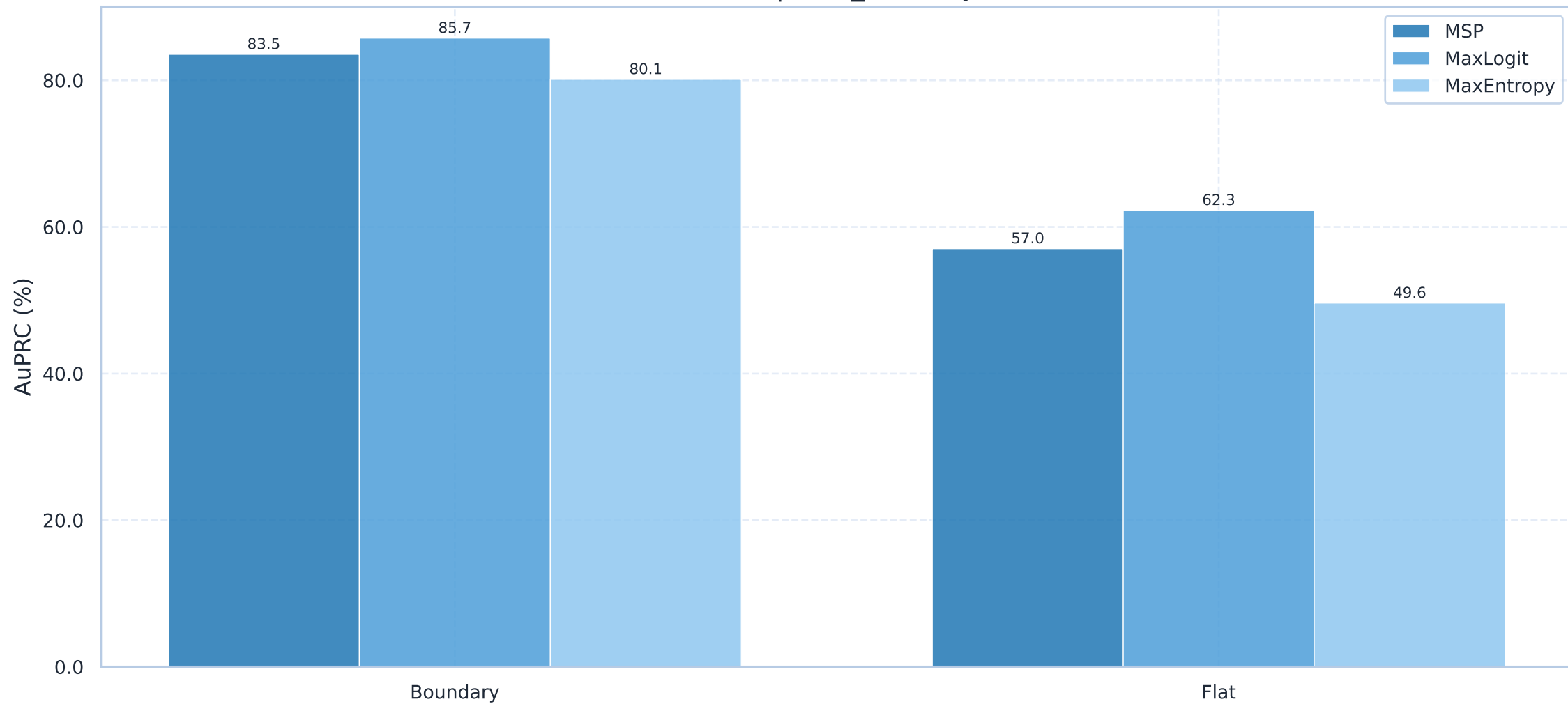
AuPRC - Boundary vs Flat Region EoMT | road_anomaly
