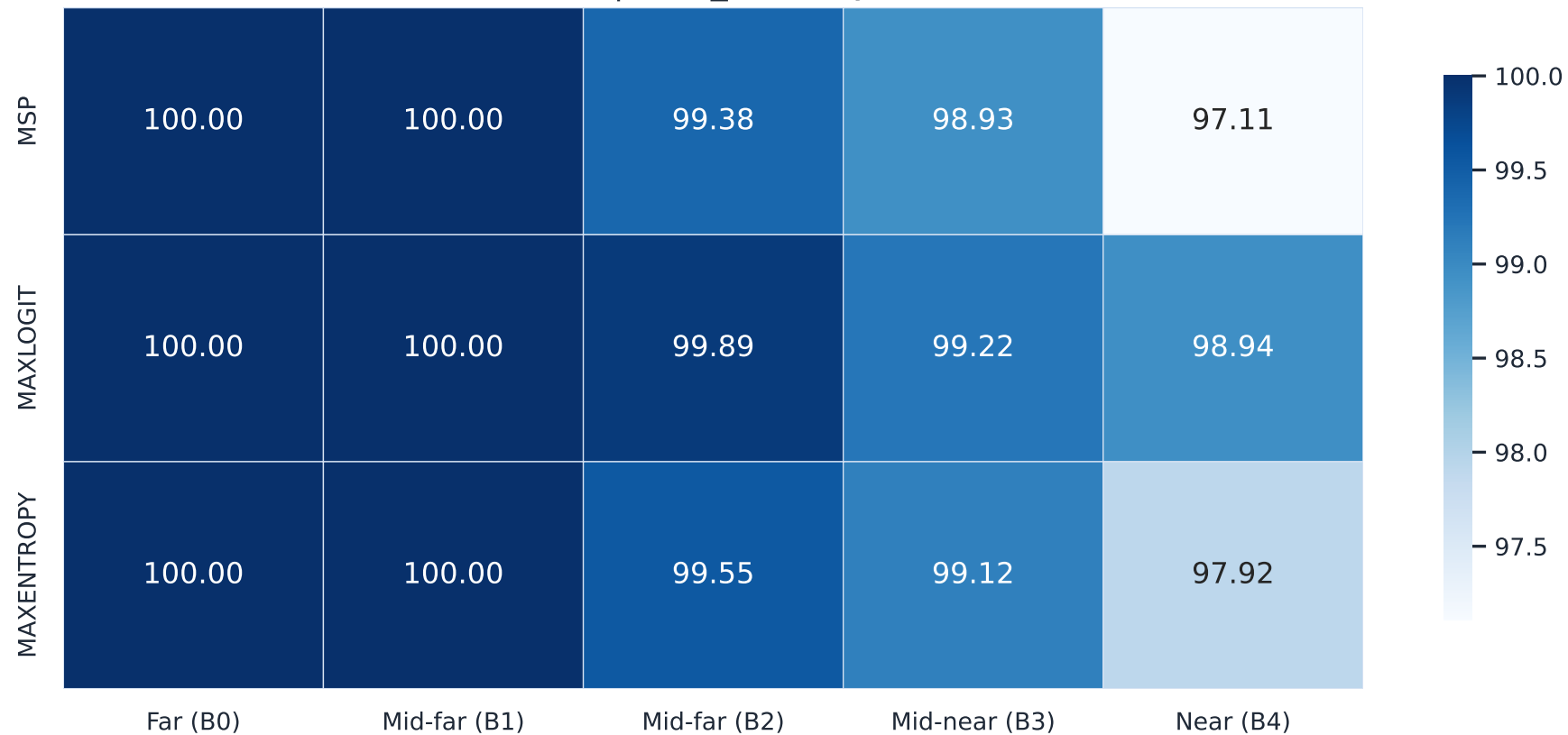
FPR@95 (%) by Depth Band EoMT | road_anomaly21
