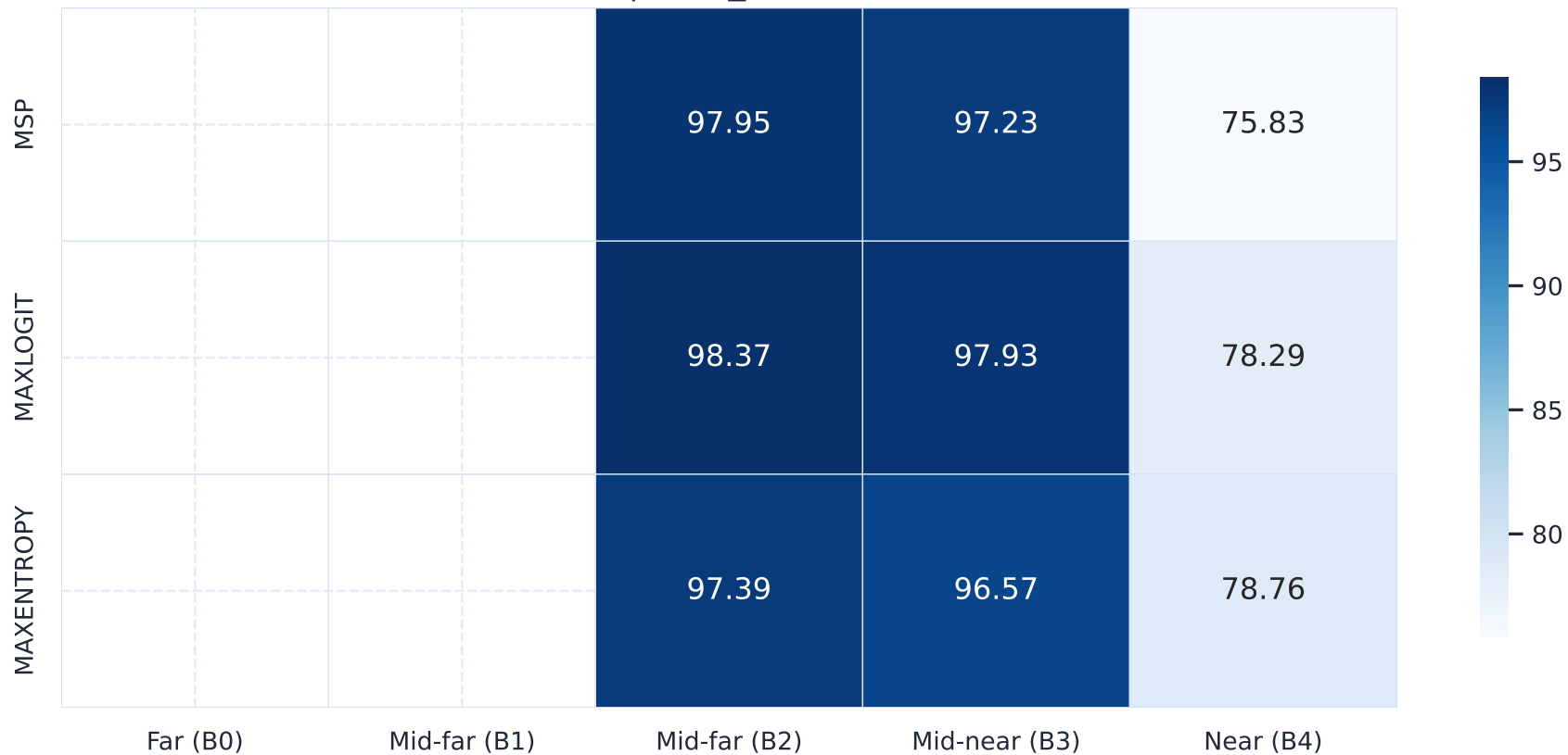
AuPRC (%) by Depth Band EoMT | road_obstacle21
