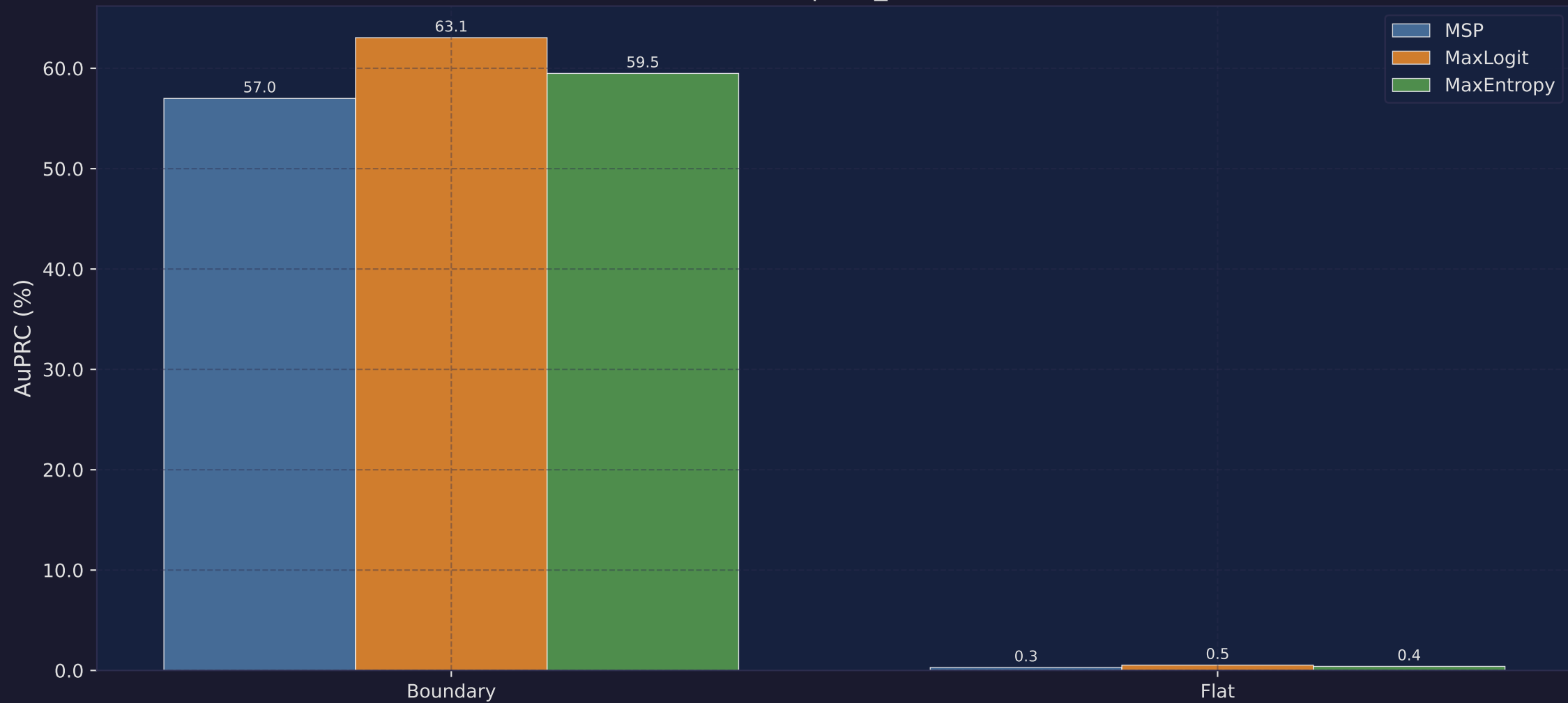
AuPRC — Boundary vs Flat Region ERFNet | lost_found
