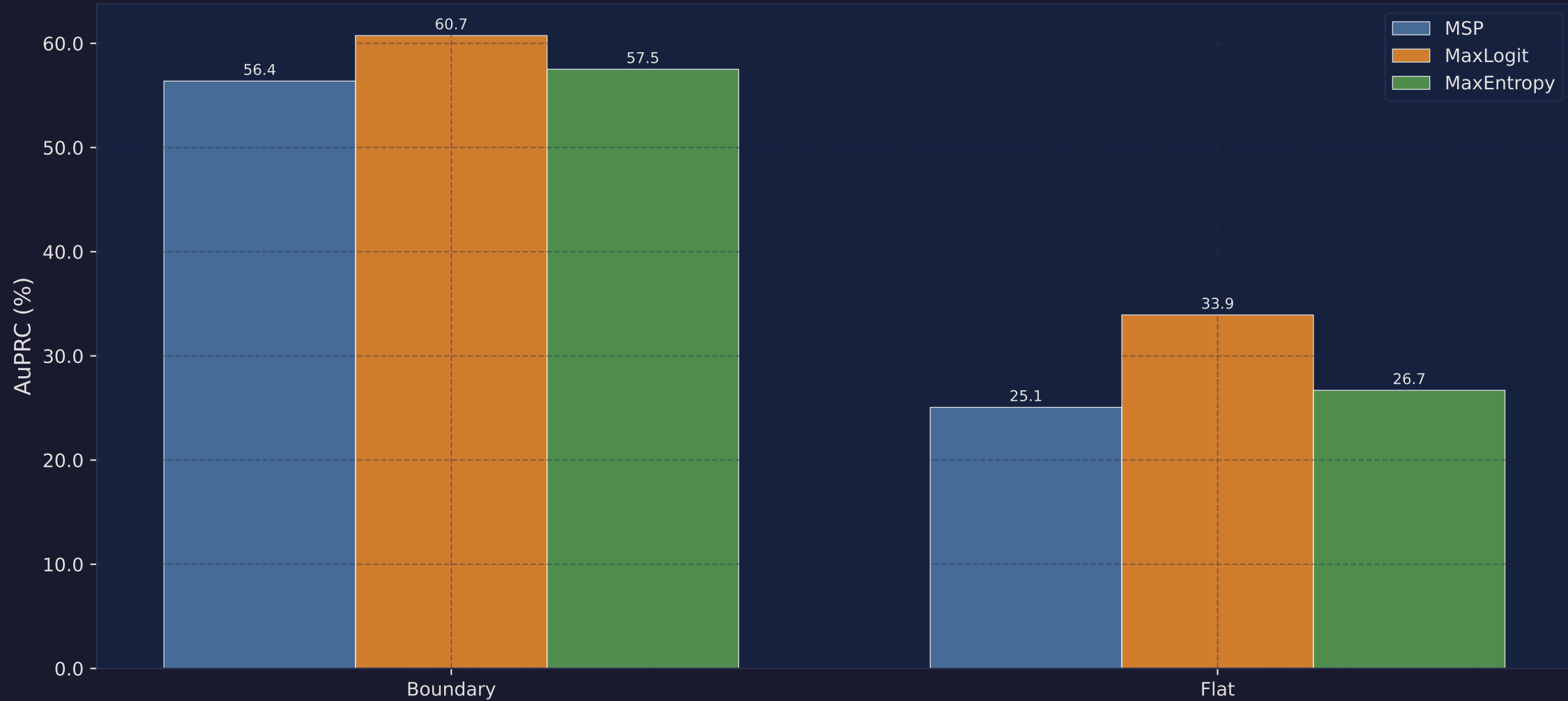
AuPRC — Boundary vs Flat Region ERFNet | road_anomaly21
