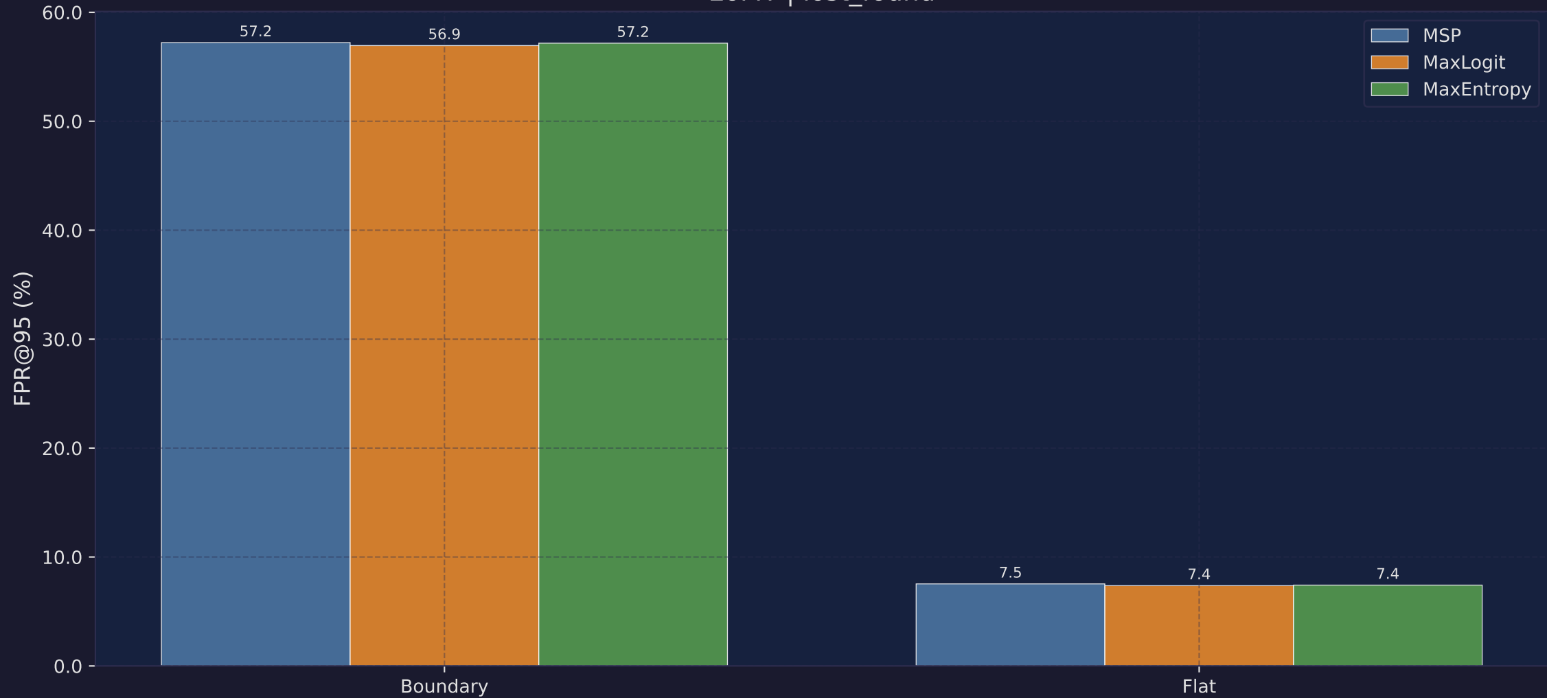
FPR@95 — Boundary vs Flat Region EoMT | lost_found
