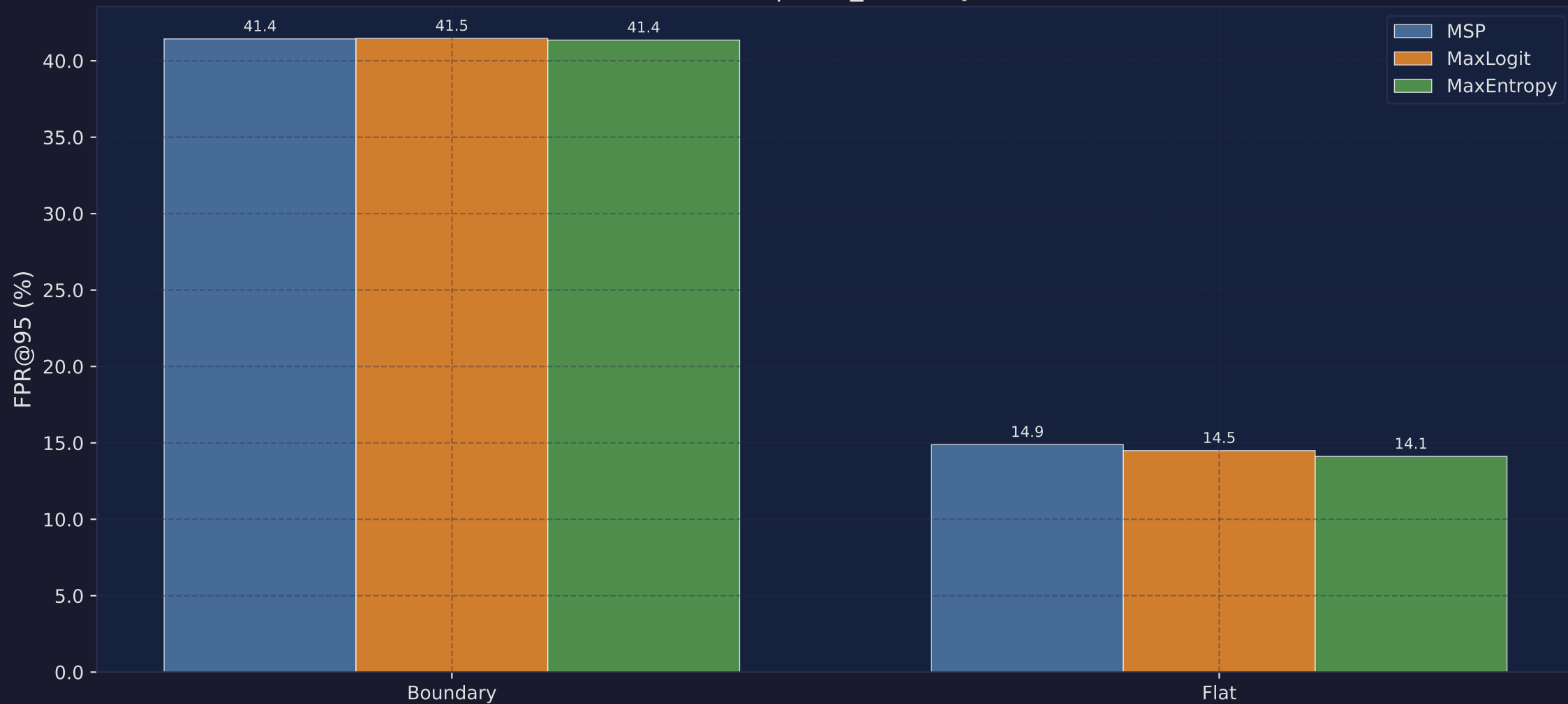
FPR@95 — Boundary vs Flat Region EoMT | road_anomaly
