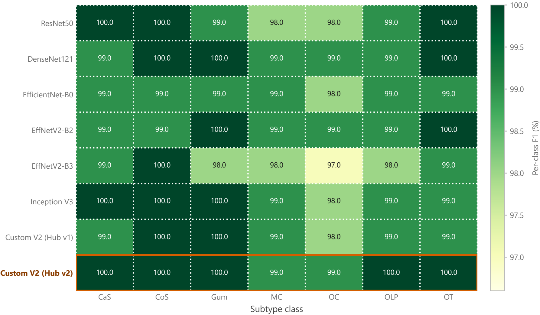
Per-class F1 score across models (Table 2a)
