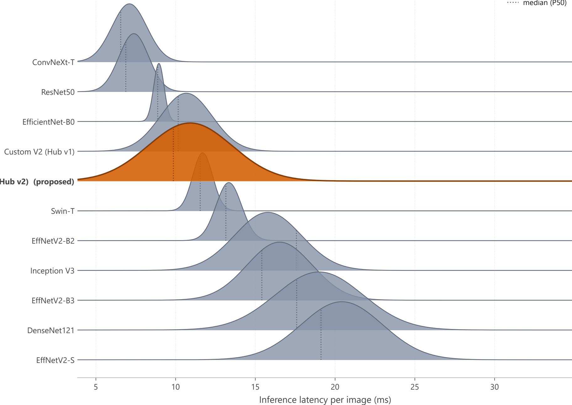
Inference latency distributions — per-model density ridgeline (lower is better)
