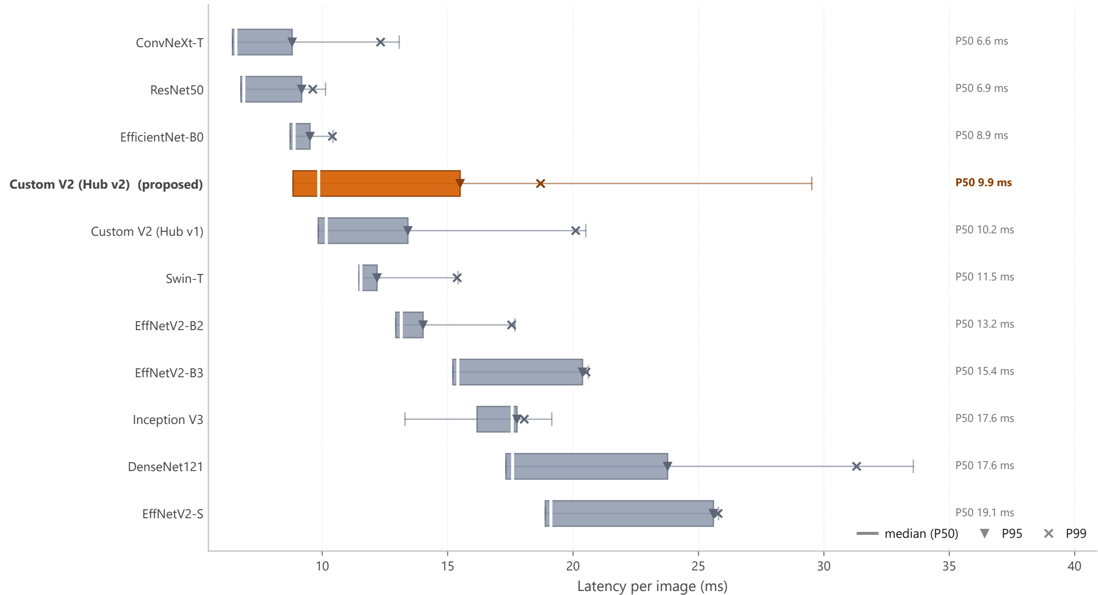
Per-model inference latency distributions
