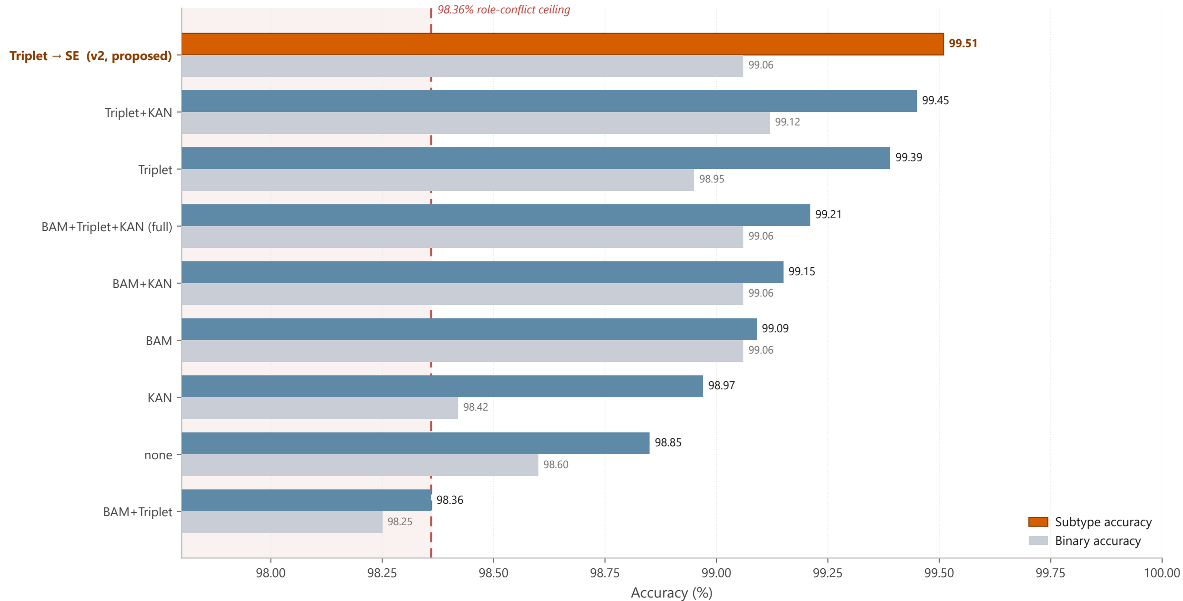
AttentionHub ablation — subtype vs. binary accuracy across variants (Table 4 + v2)
