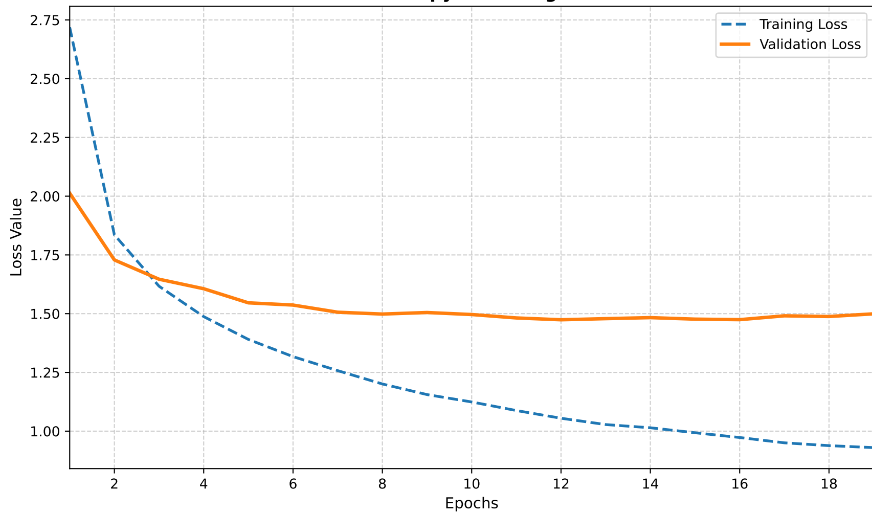
Cross-Entropy Loss Progression
