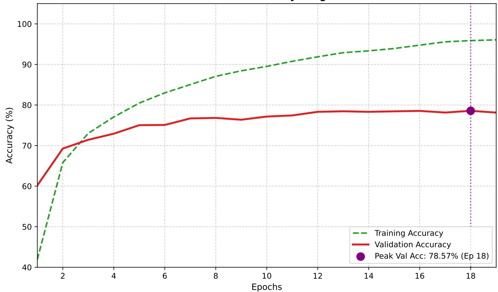
Classification Accuracy Progression
