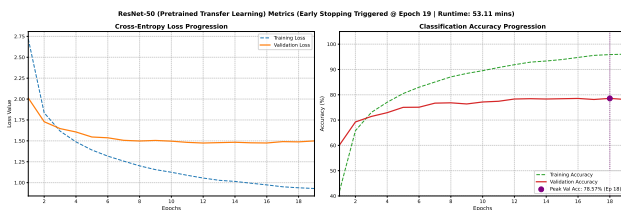
Figure 8: Training and validation metrics for the Step 6 Pre-trained ResNet-50 Transfer Learning model[cite: 8].
