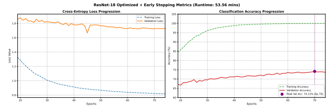
Figure 5: Training and validation metrics for the Step 3 Custom Topographic Patch ResNet-18[cite: 4].
