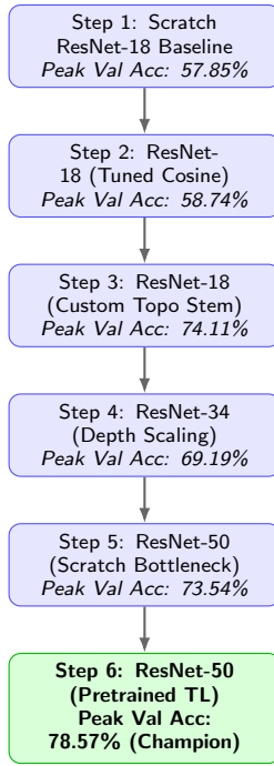
Figure 2: Chronological experimental flow diagram illustrating the 6-step diagnostic progression[cite: 1].
