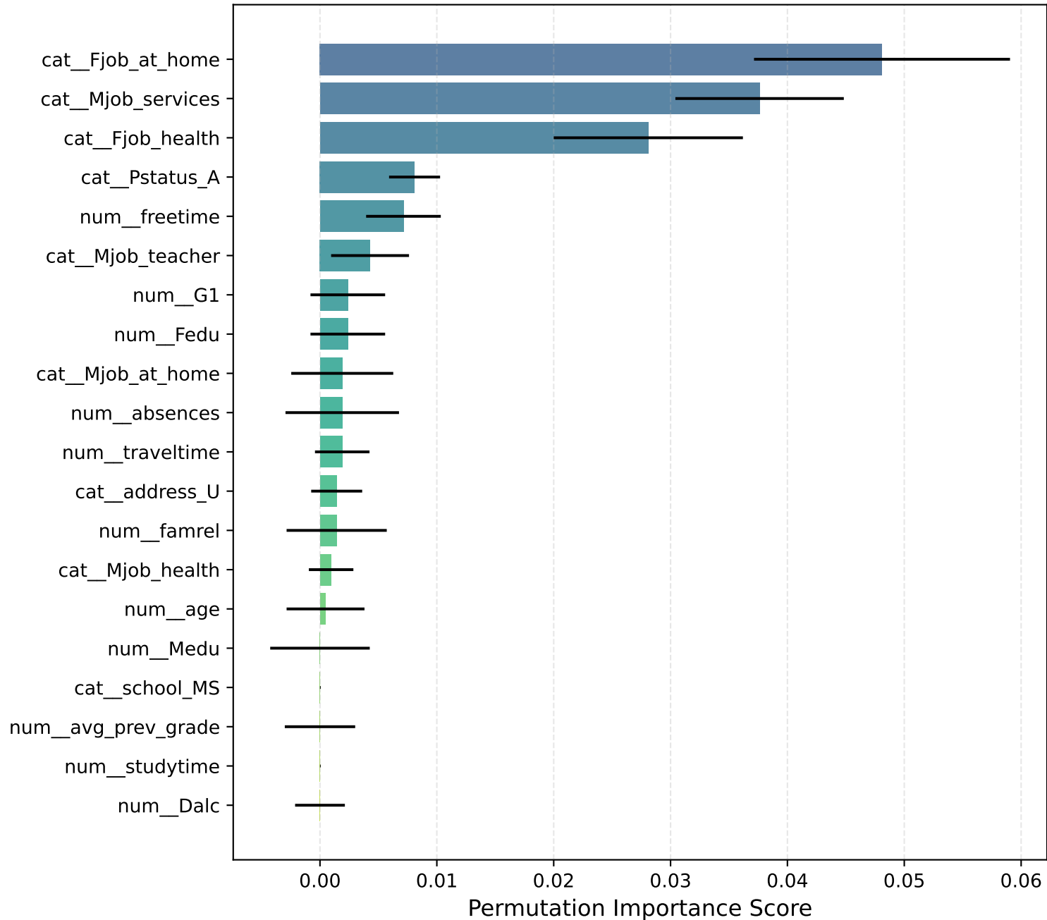
Top 20 Features by Permutation Importance
