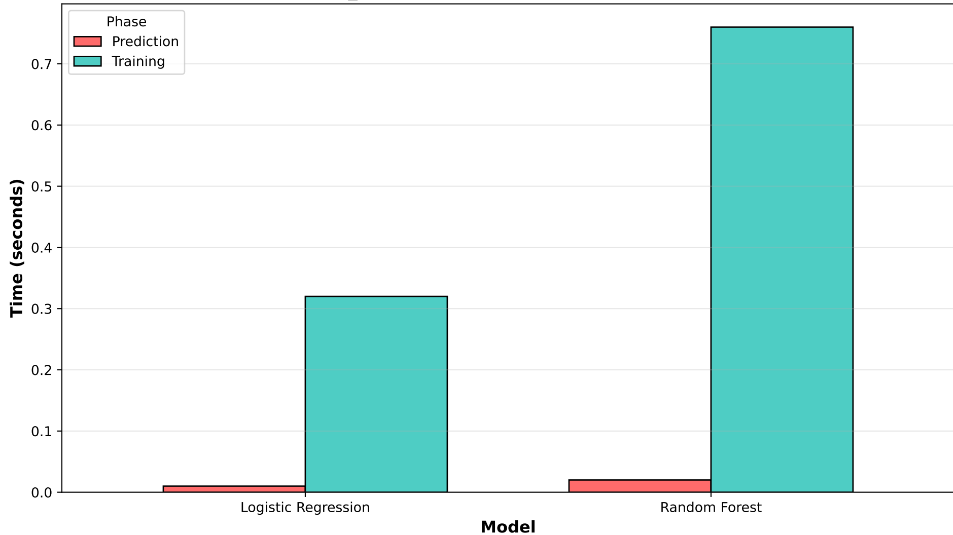
RQ4_Fig4: Model Runtime Comparison
