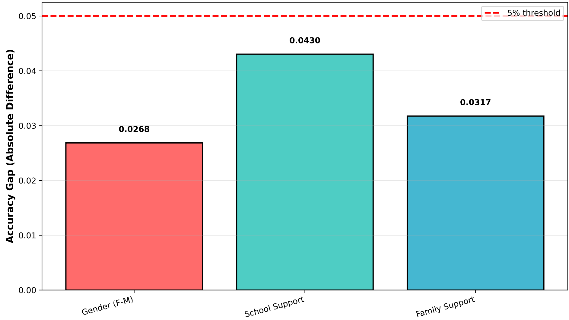
RQ3_Fig4: Fairness Gap Analysis
