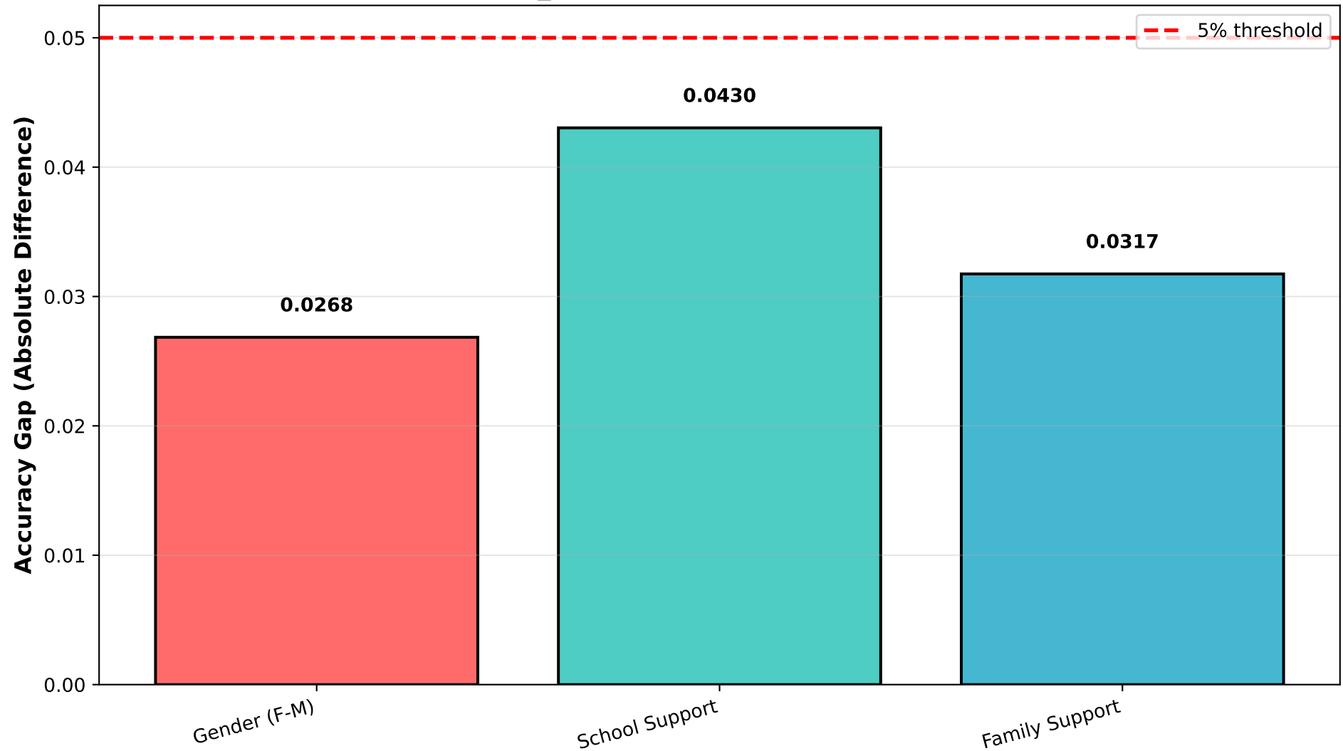
RQ3_Fig4: Fairness Gap Analysis
