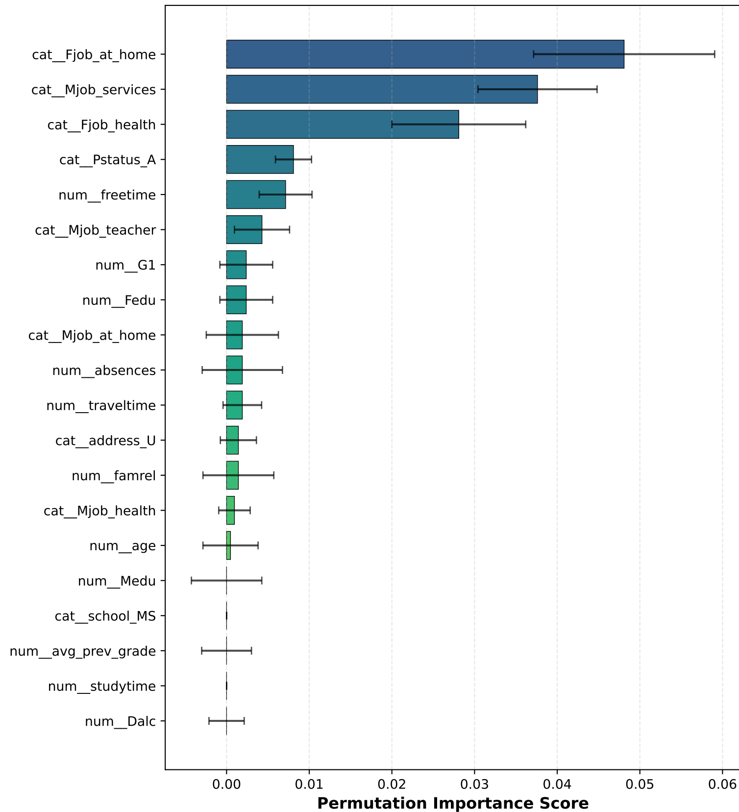
Top 20 Features by Permutation Importance
