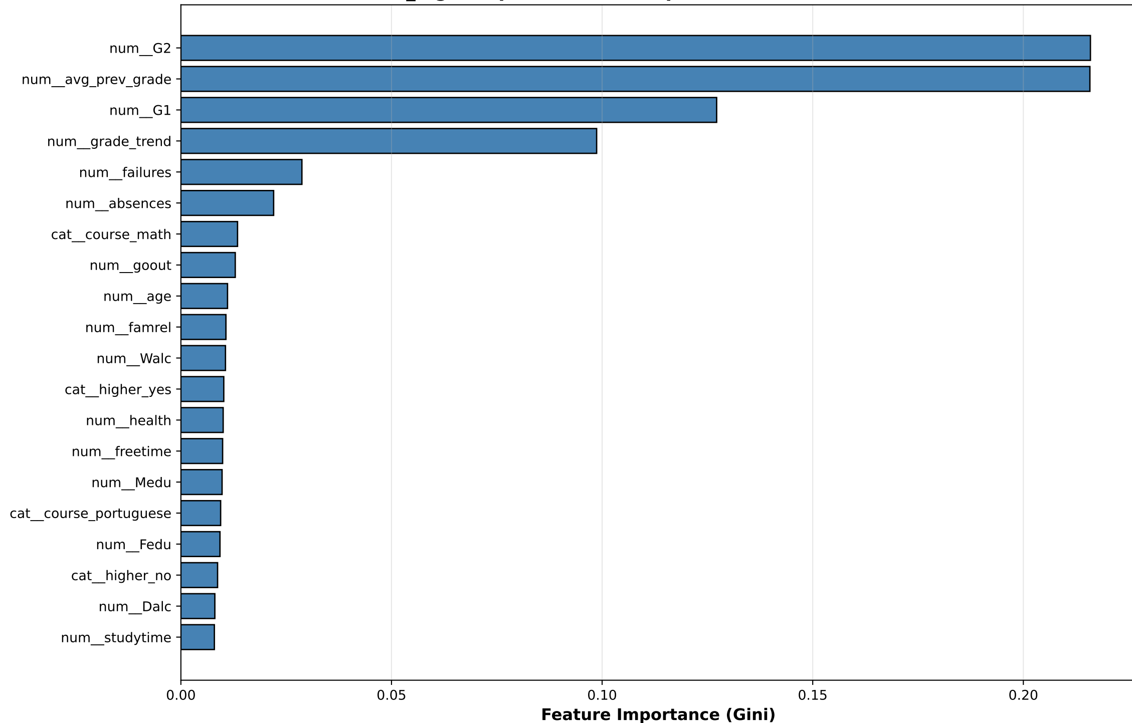
RQ4_Fig1: Top 20 Feature Importances (Random Forest)
