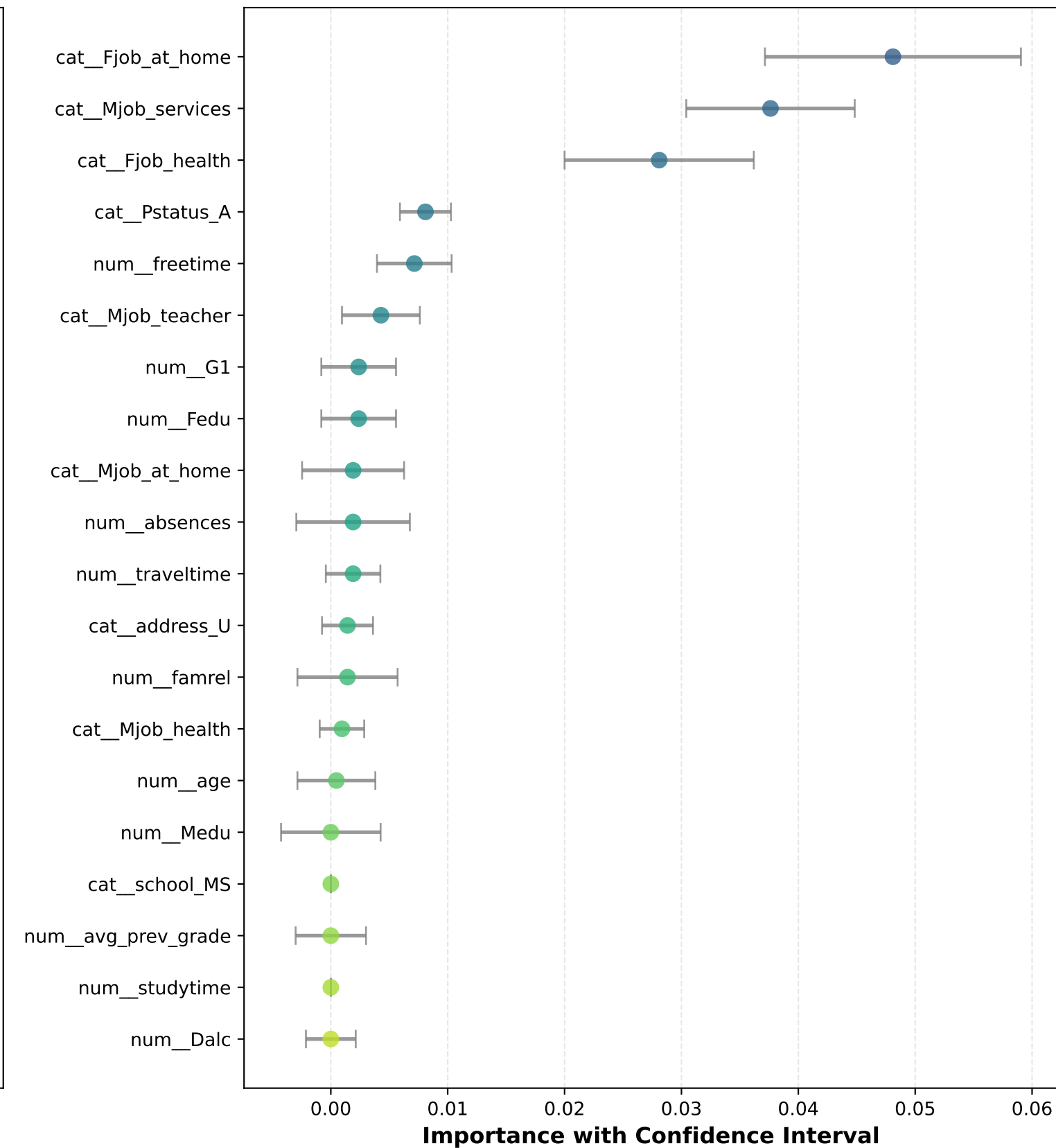
Feature Importance Uncertainty
