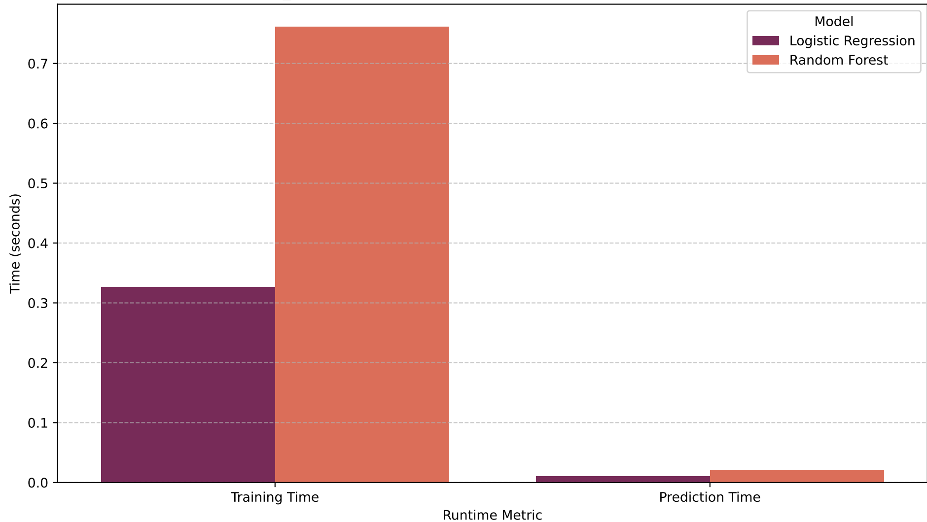
RQ4_Fig4: Model Runtime Comparison: Training vs. Prediction
