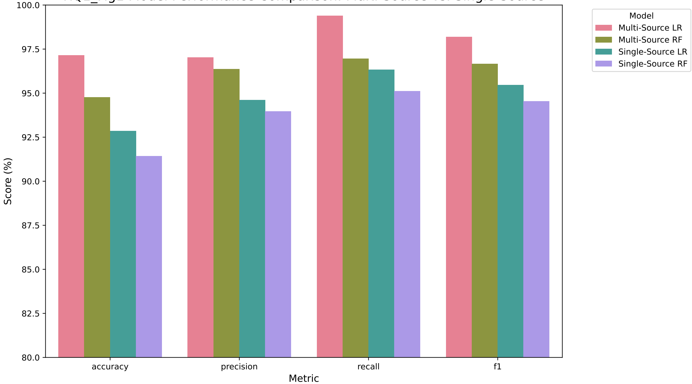
RQ1_Fig1 Model Performance Comparison: Multi-Source vs. Single-Source
