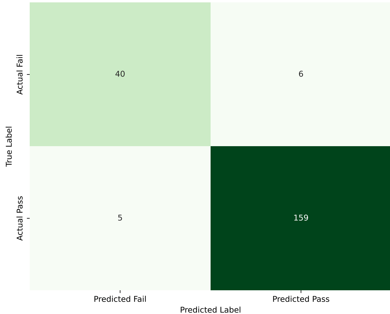
Random Forest Confusion Matrix
