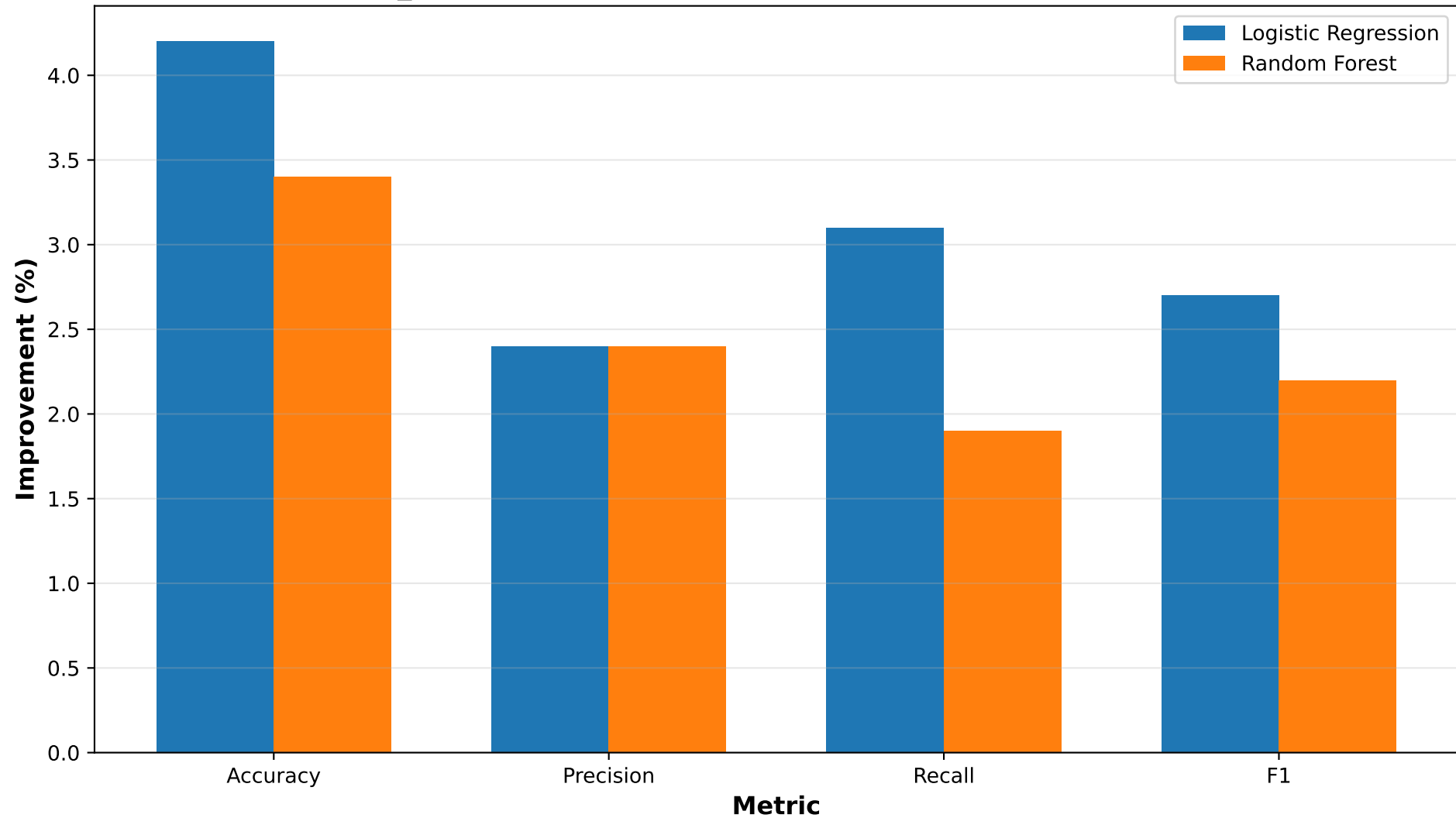
RQ1_Fig3: Multi-Source vs Single-Source Improvement
