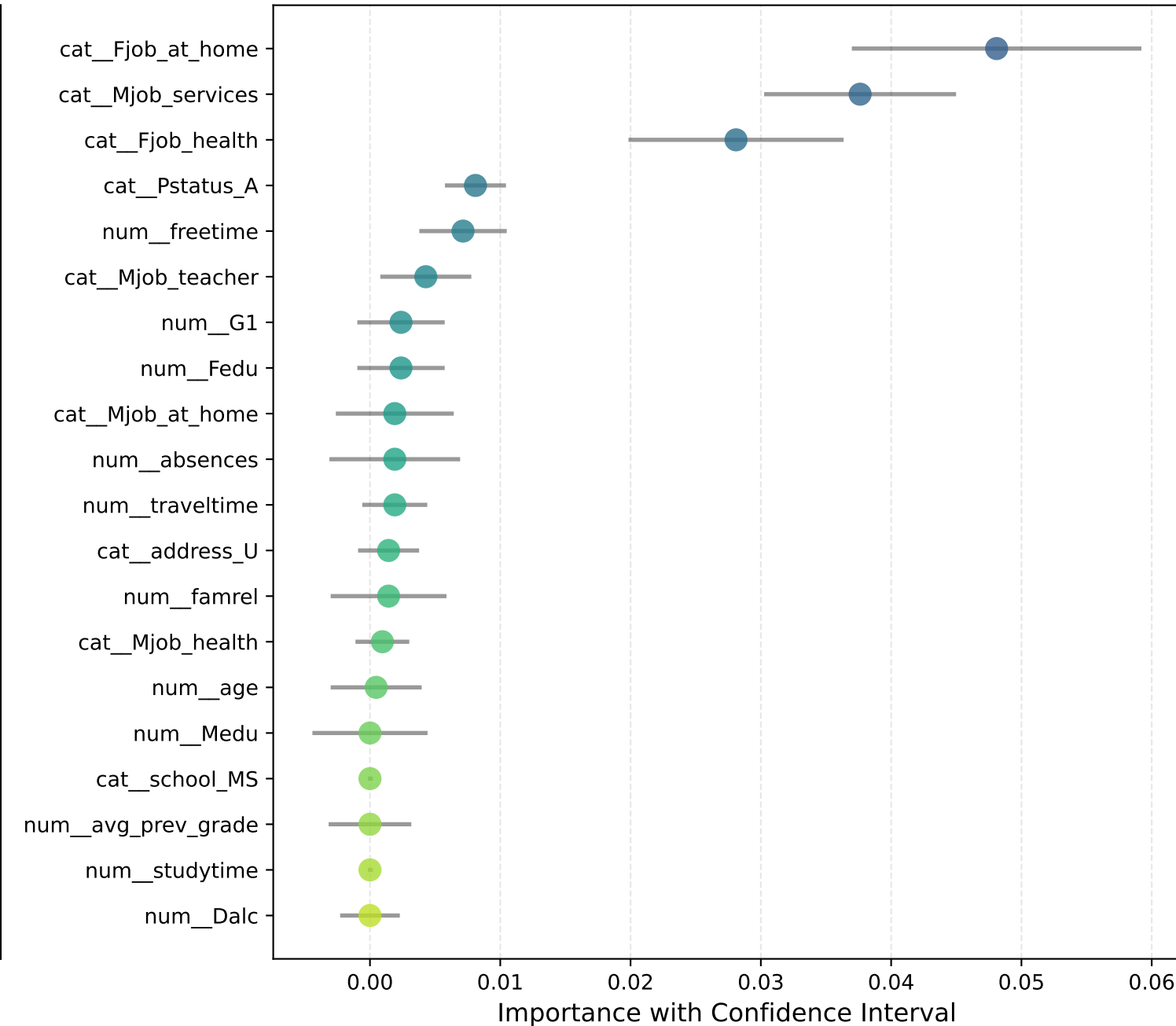
Feature Importance Uncertainty
