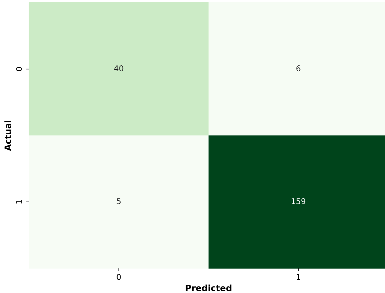
Random Forest
