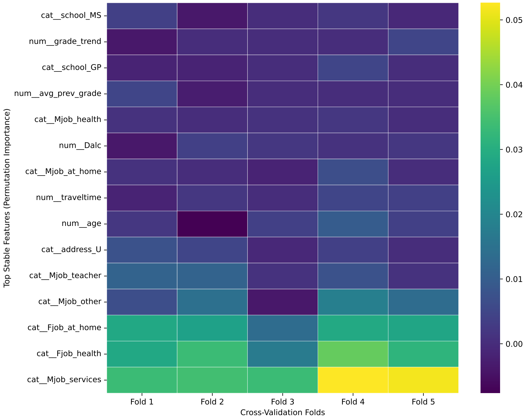
RQ4_Fig1: Feature Stability Map Across Cross-Validation Folds
