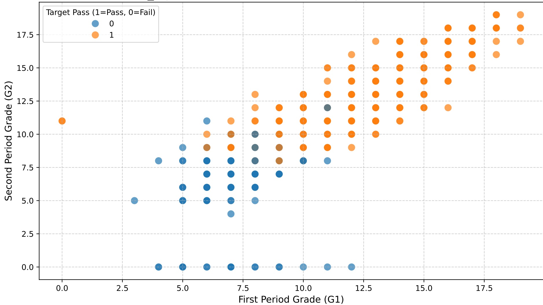
RQ1_Fig2 G1 vs G2 Grades, Colored by Pass/Fail Status
