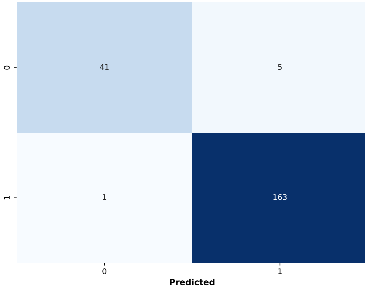
Logistic Regression
