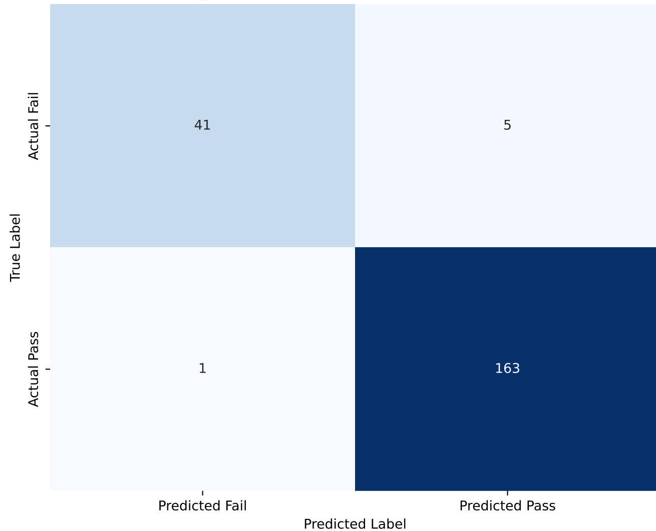
RQ4_Fig3: Logistic Regression Confusion Matrix
