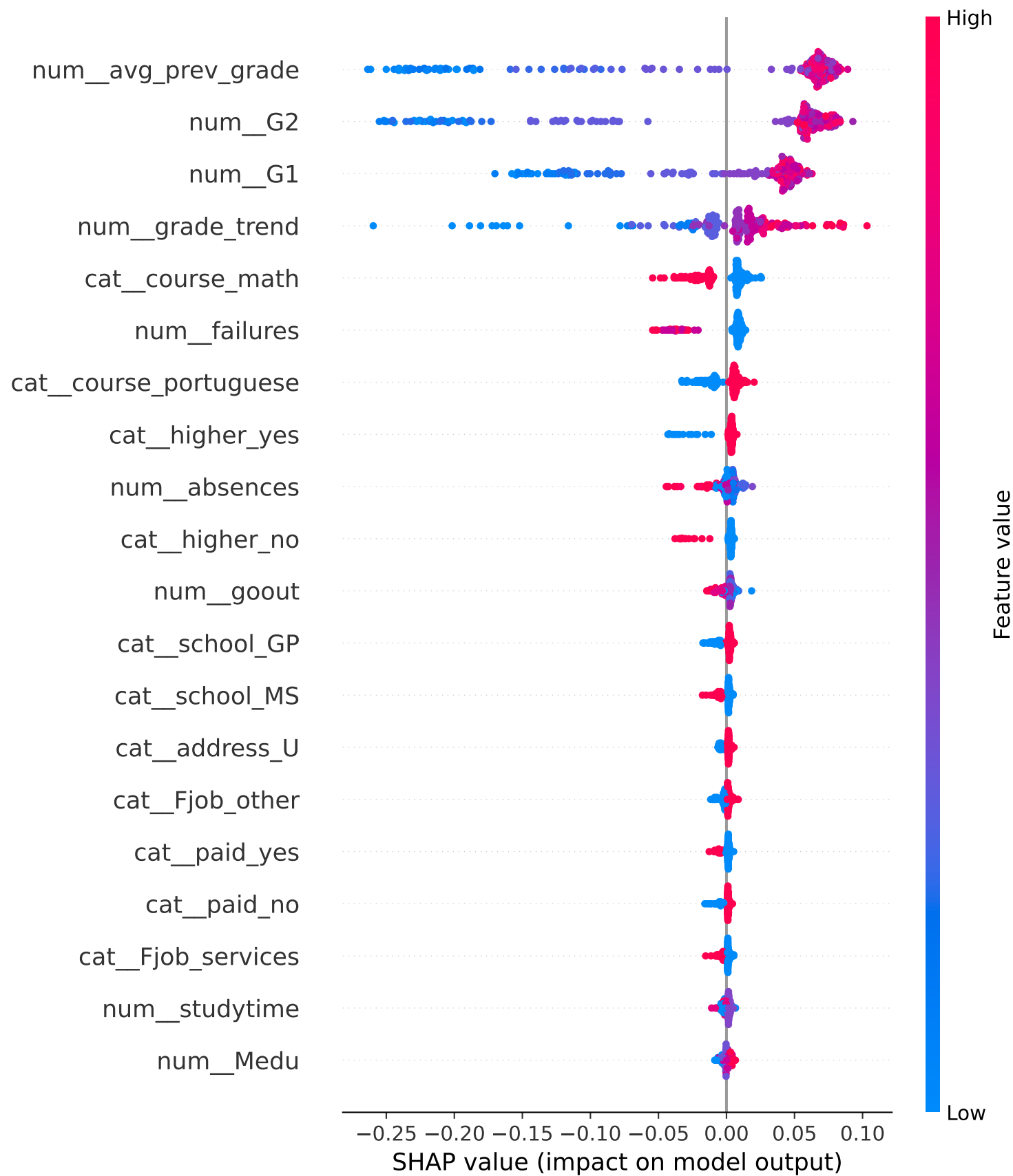
RQ4_Fig6: SHAP Value Distribution for Academic Performance (Random Forest)
