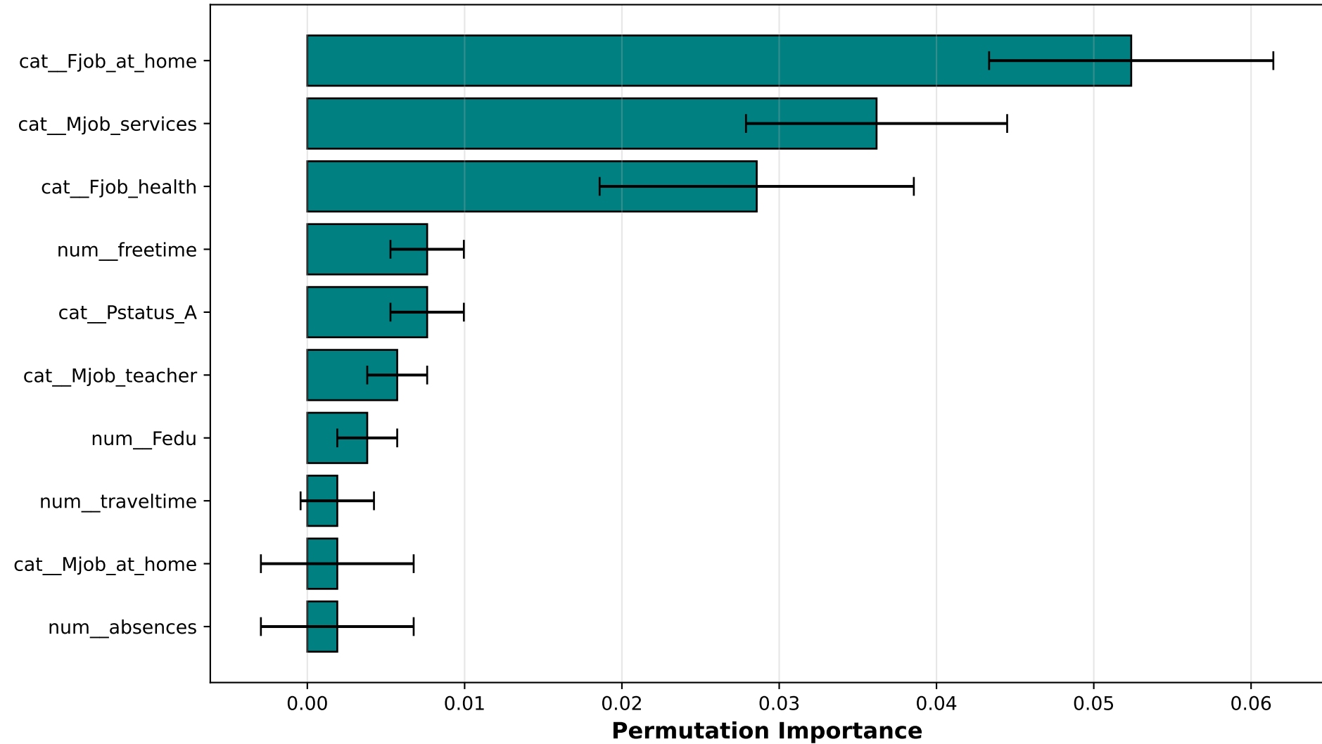
RQ4_Fig5: Top 10 Features by Permutation Importance
