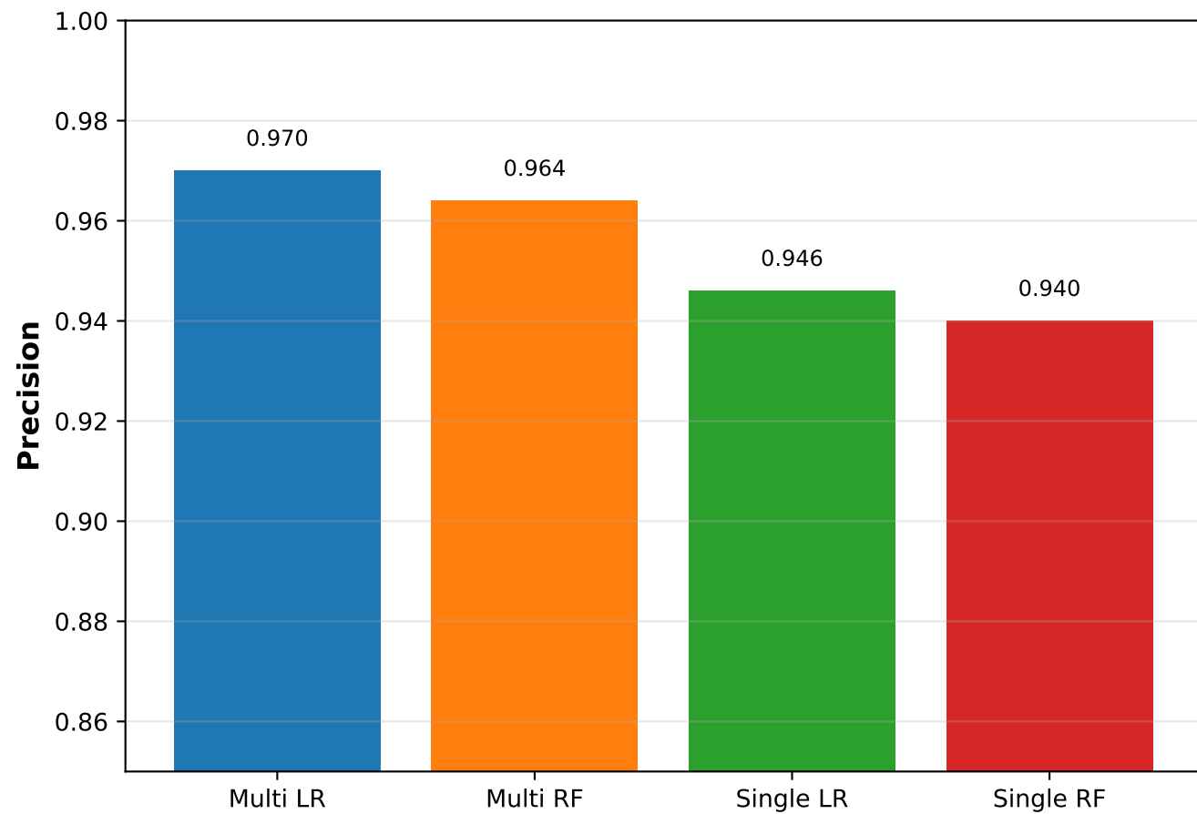
RQ1_Fig1: Model Performance Comparison
