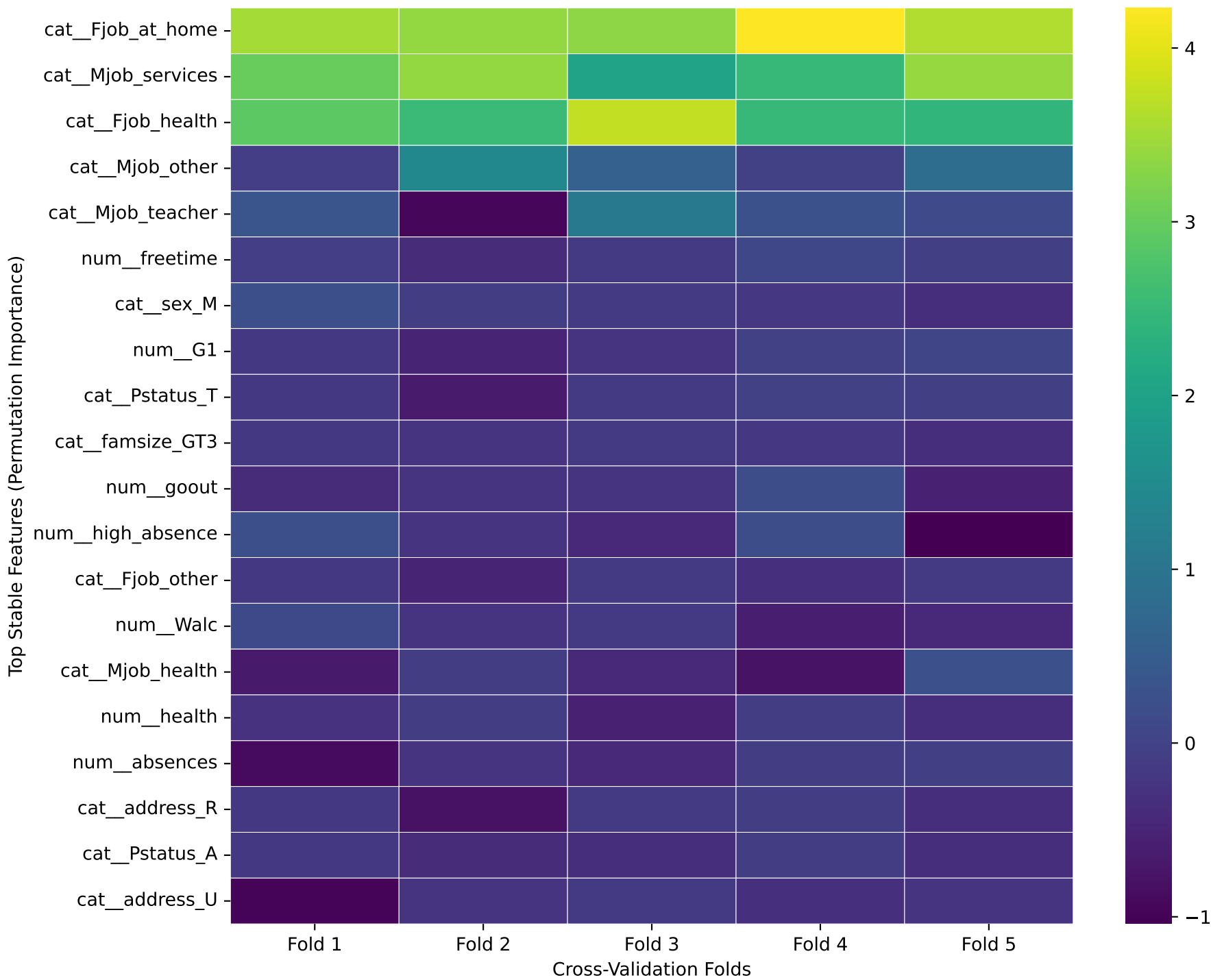
RQ4_Fig1: Feature Stability Map Across Cross-Validation Folds
