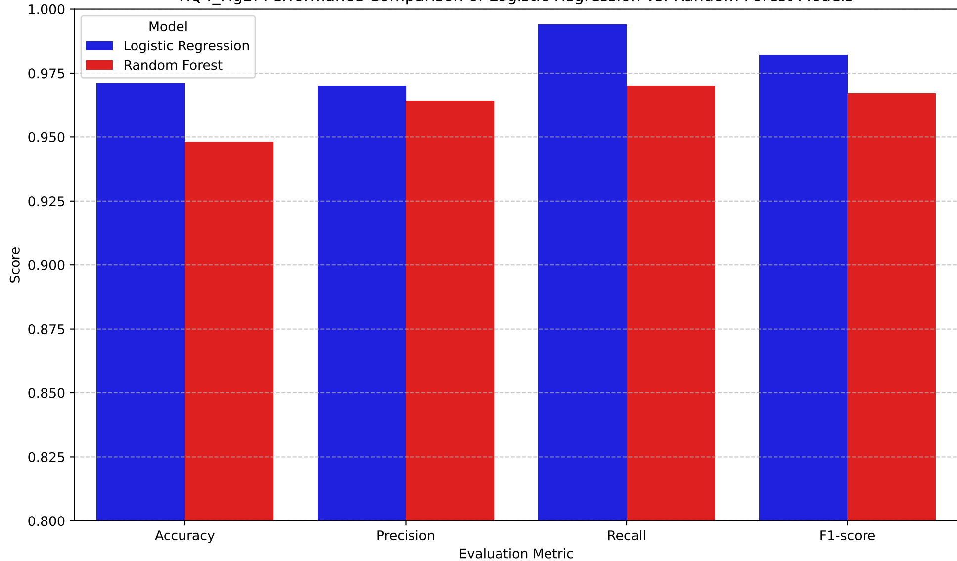
RQ4_Fig2: Performance Comparison of Logistic Regression vs. Random Forest Models
