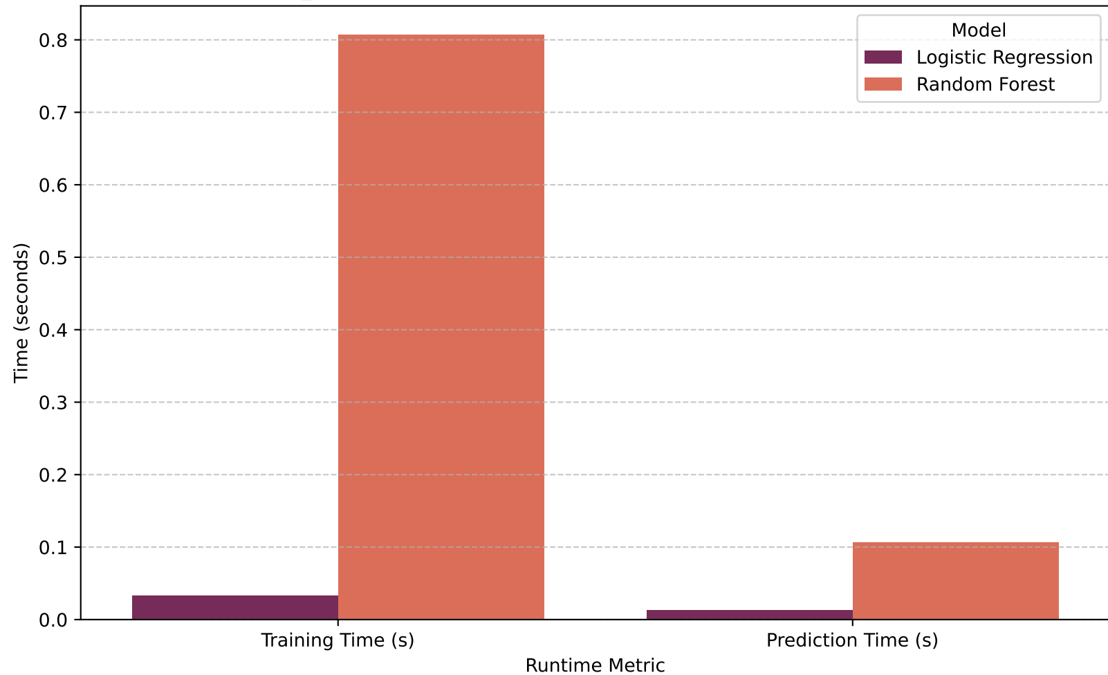
RQ4_Fig4: Model Runtime Comparison: Training vs. Prediction
