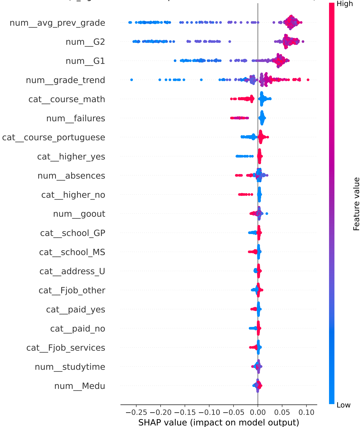
RQ4_Fig6: SHAP Feature Importance for Academic Performance (Random Forest)
