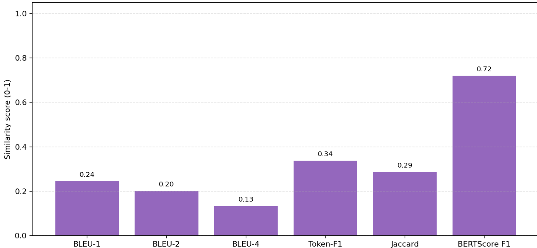
Answer vs Reference Semantic Similarity
