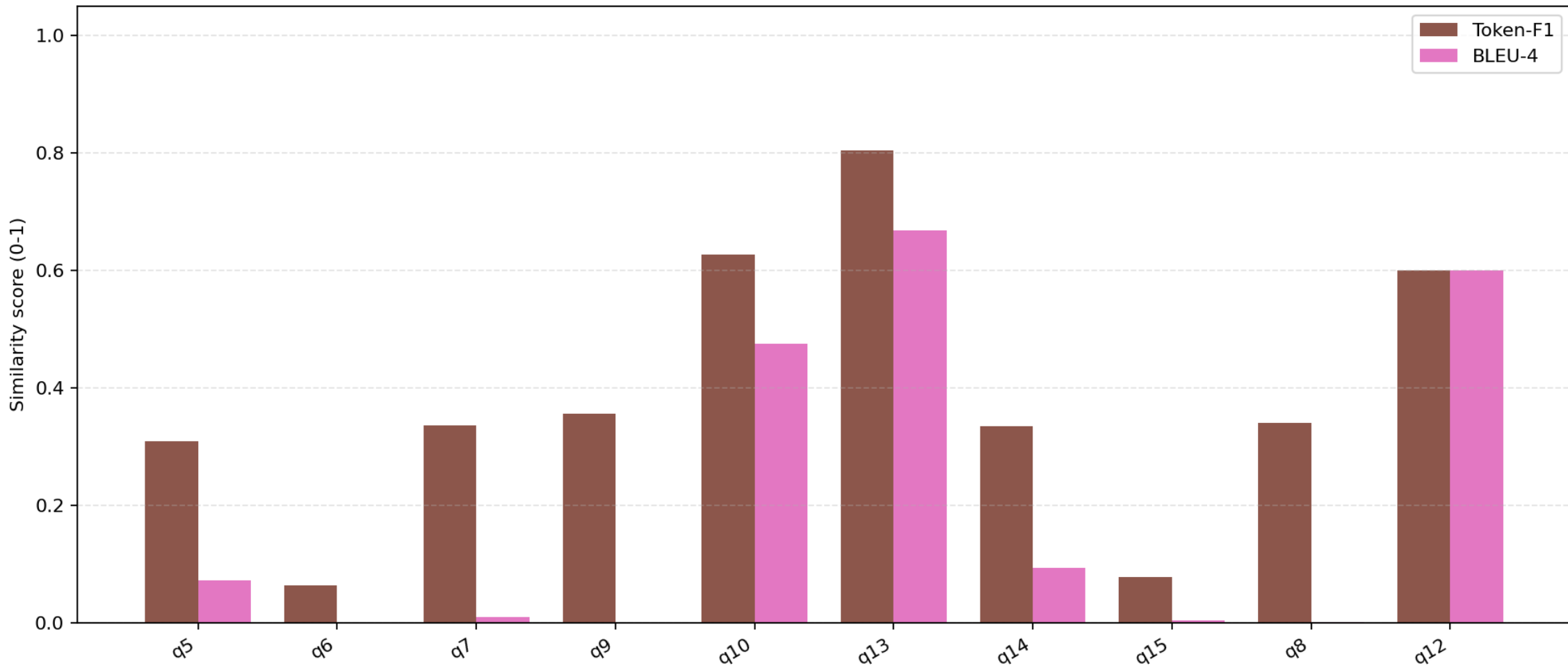
Answer vs Reference Similarity by Question
