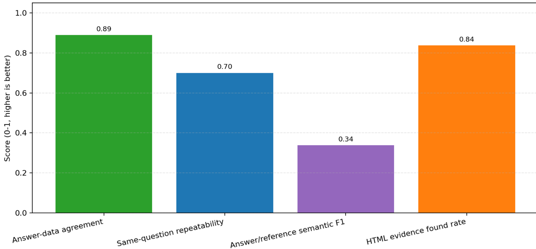
Overall Evaluation Scores
