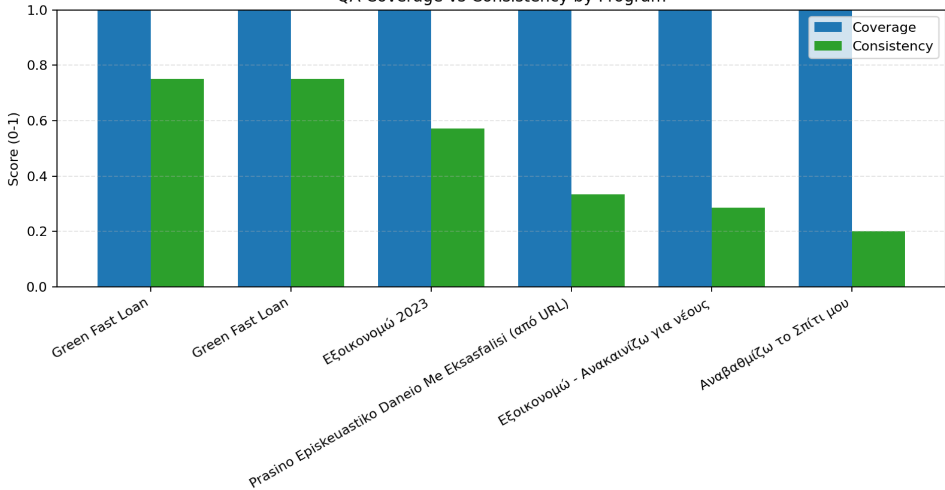
QA Coverage vs Consistency by Program
