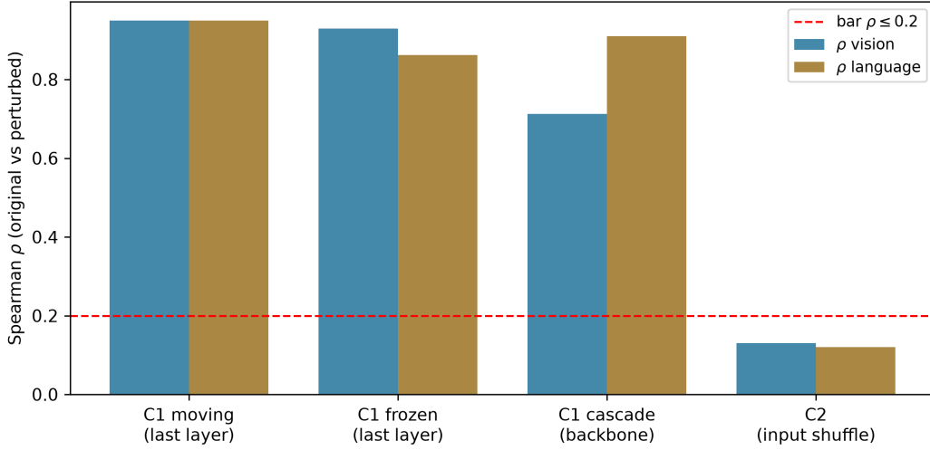
Figure 6: Historical model-randomization correlations. Frozen-reference and cascade values use saved records; standard C1 and C2 preserve unavailable original summaries. Variants change randomized parameters and may differ in source contexts or budgets. Persistent correlation does not uniquely identify input anchoring; low C2 correlation does not establish learned-model dependence.
