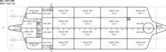
DOUBLE BOTTOM At 300mm from B.L.
