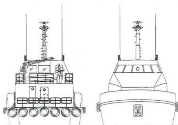
STERN VIEW
