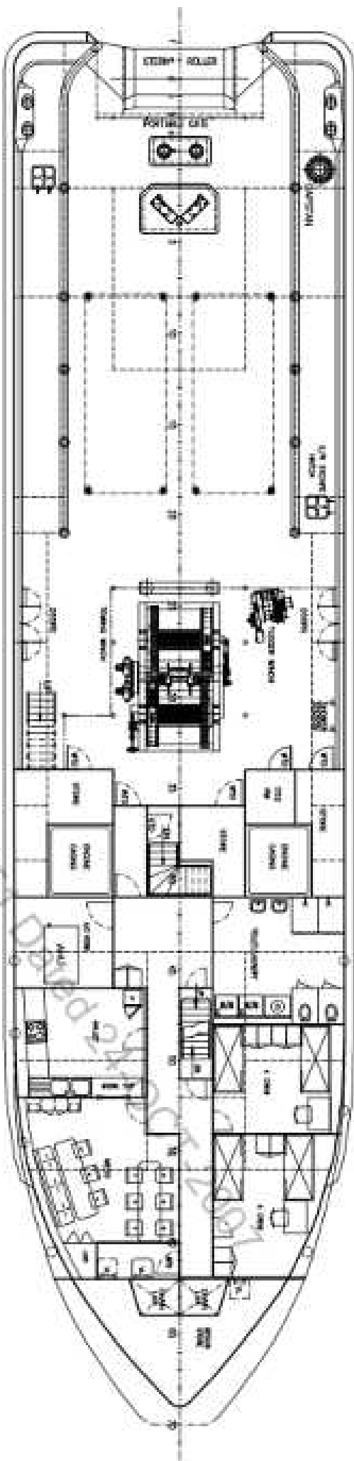
MAIN DECK PLAN
