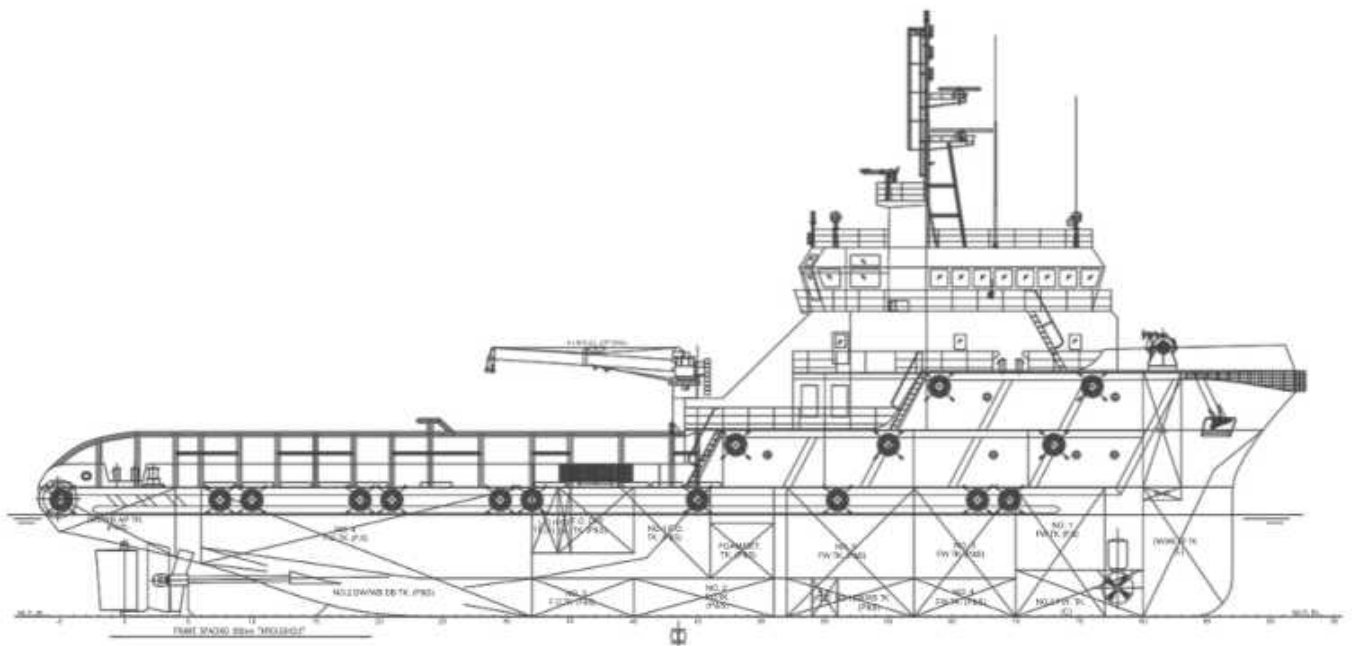
Outboard profile
