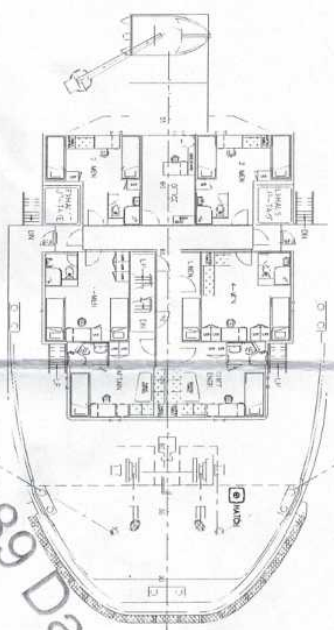
UPPER F.C. DECK
