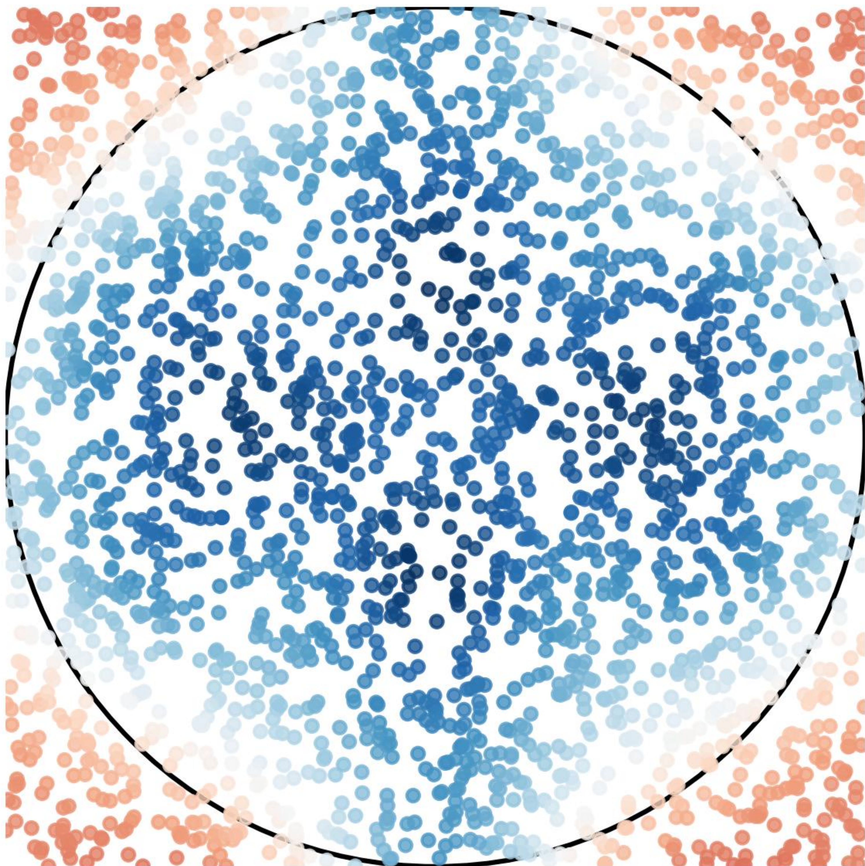
Noiseless
