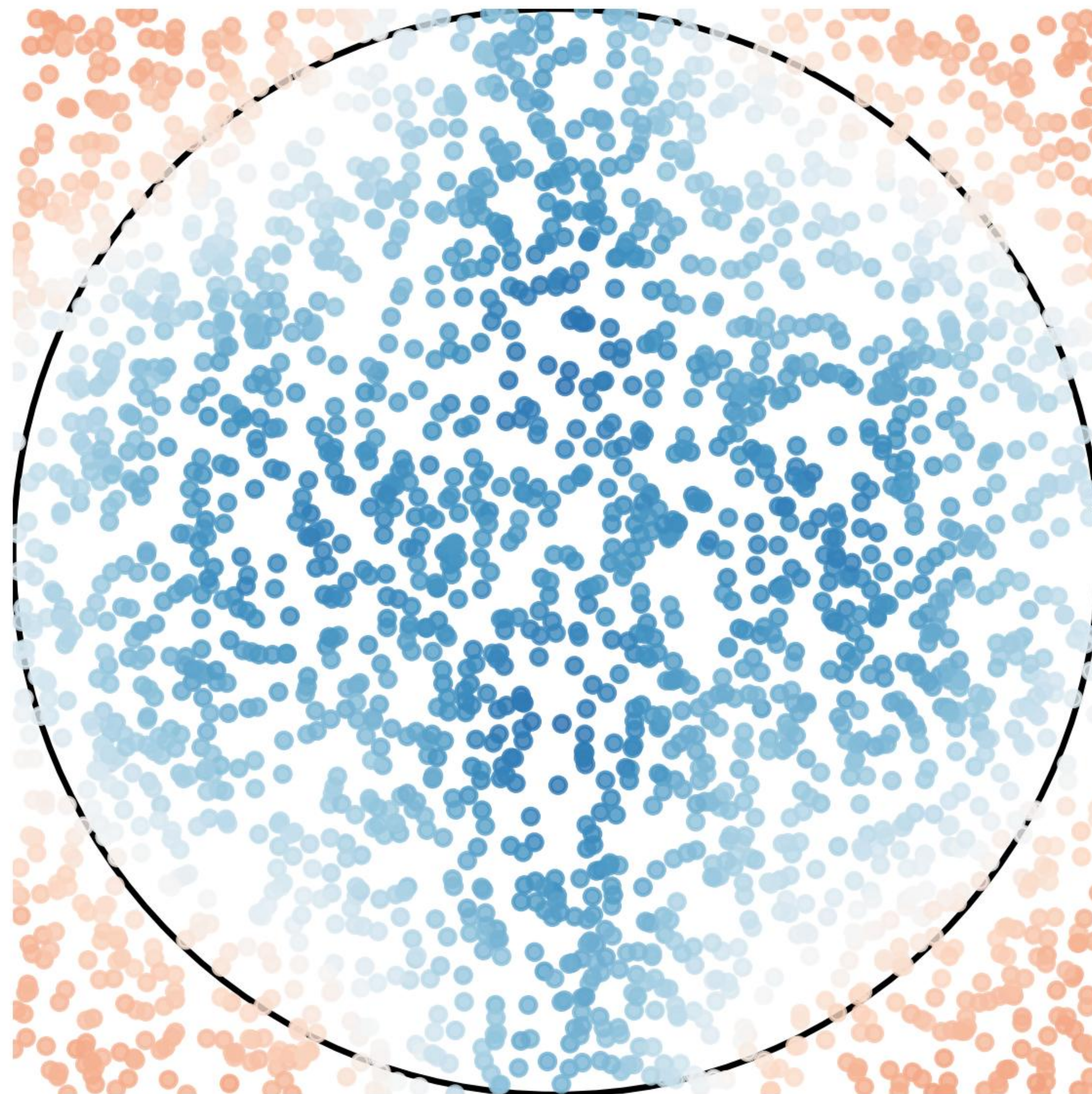
Noisy 0.005
