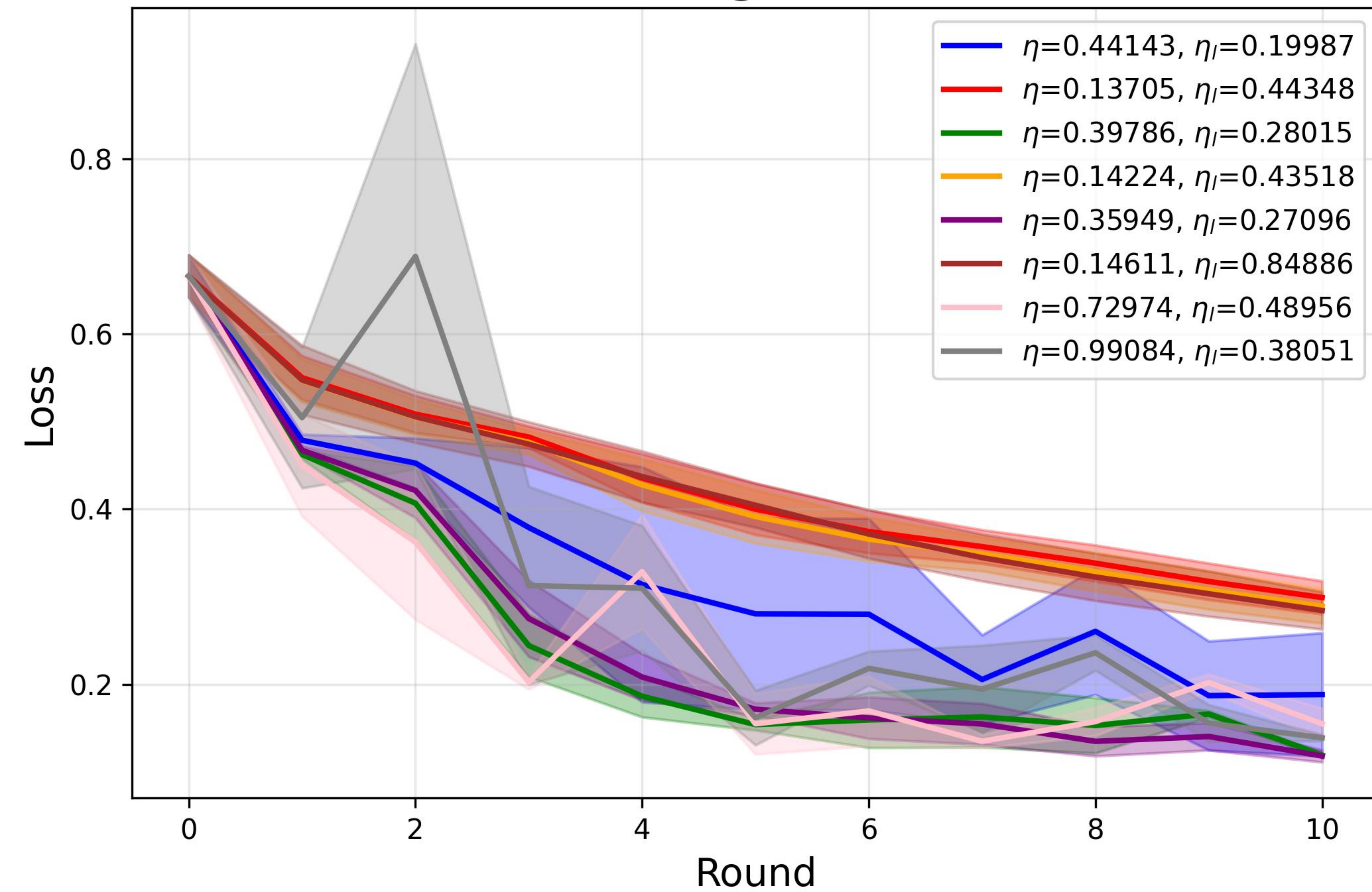
FedAdagrad Loss
