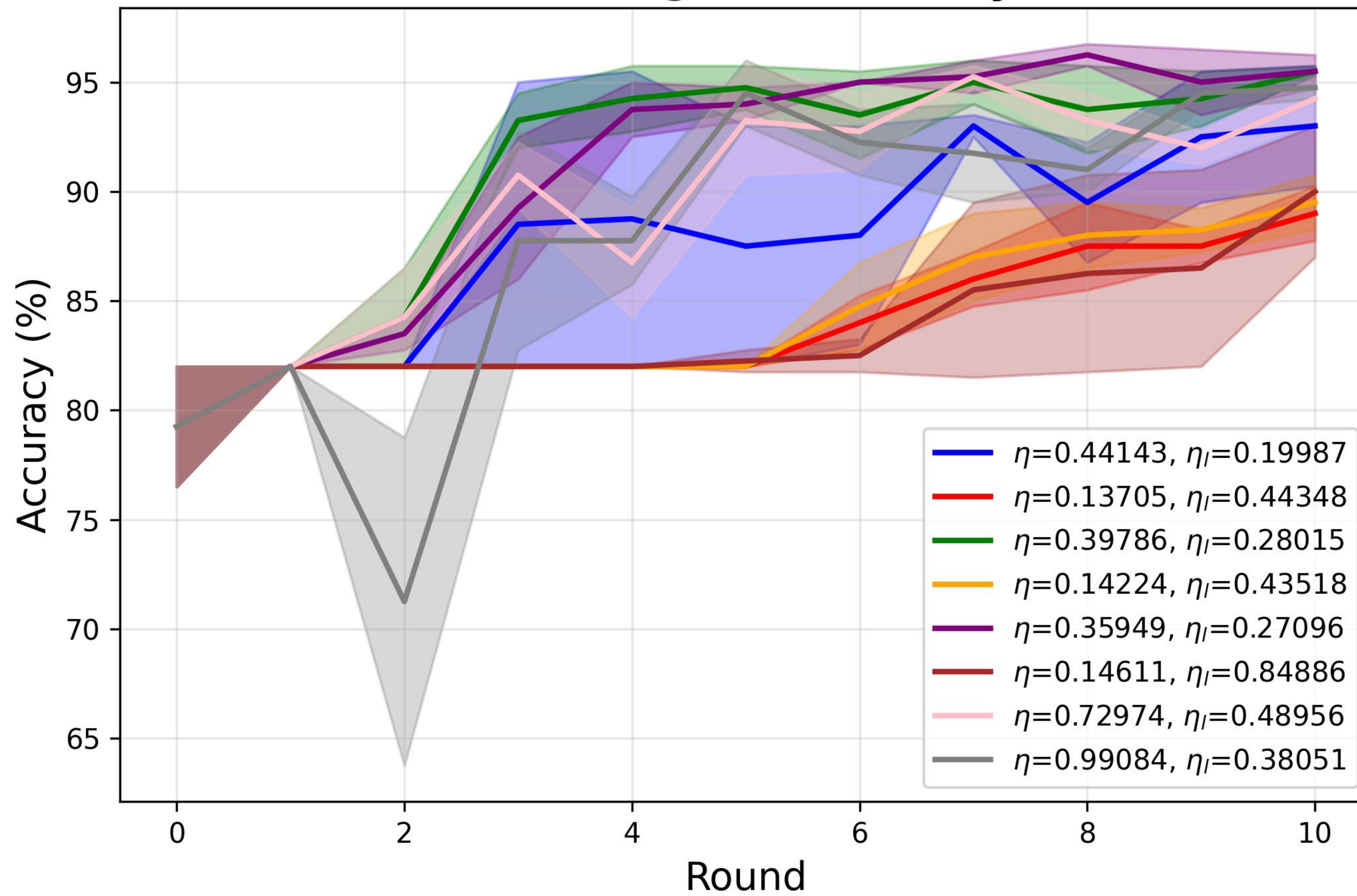
FedAdagrad Accuracy
