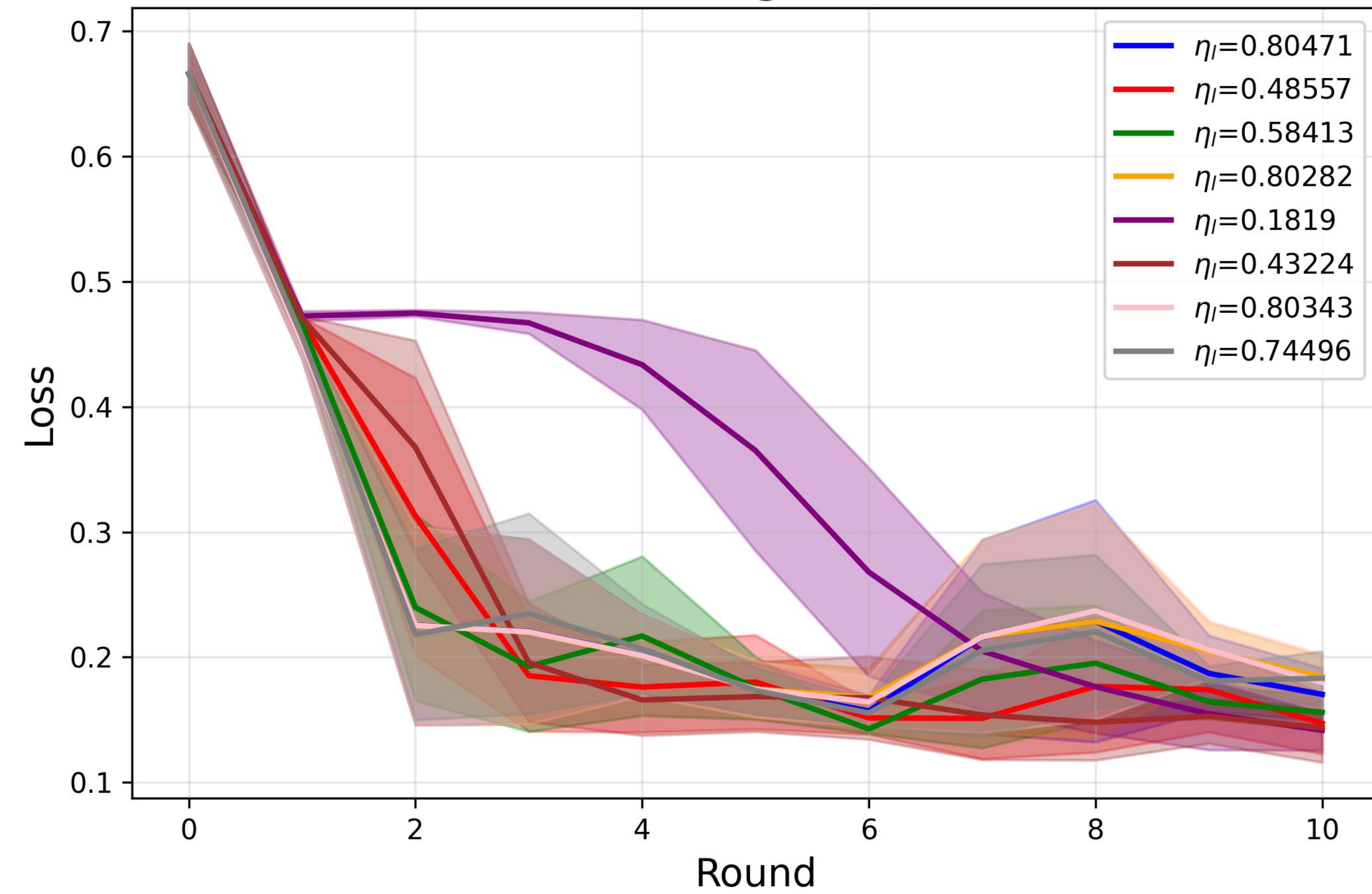
FedAvg Loss
