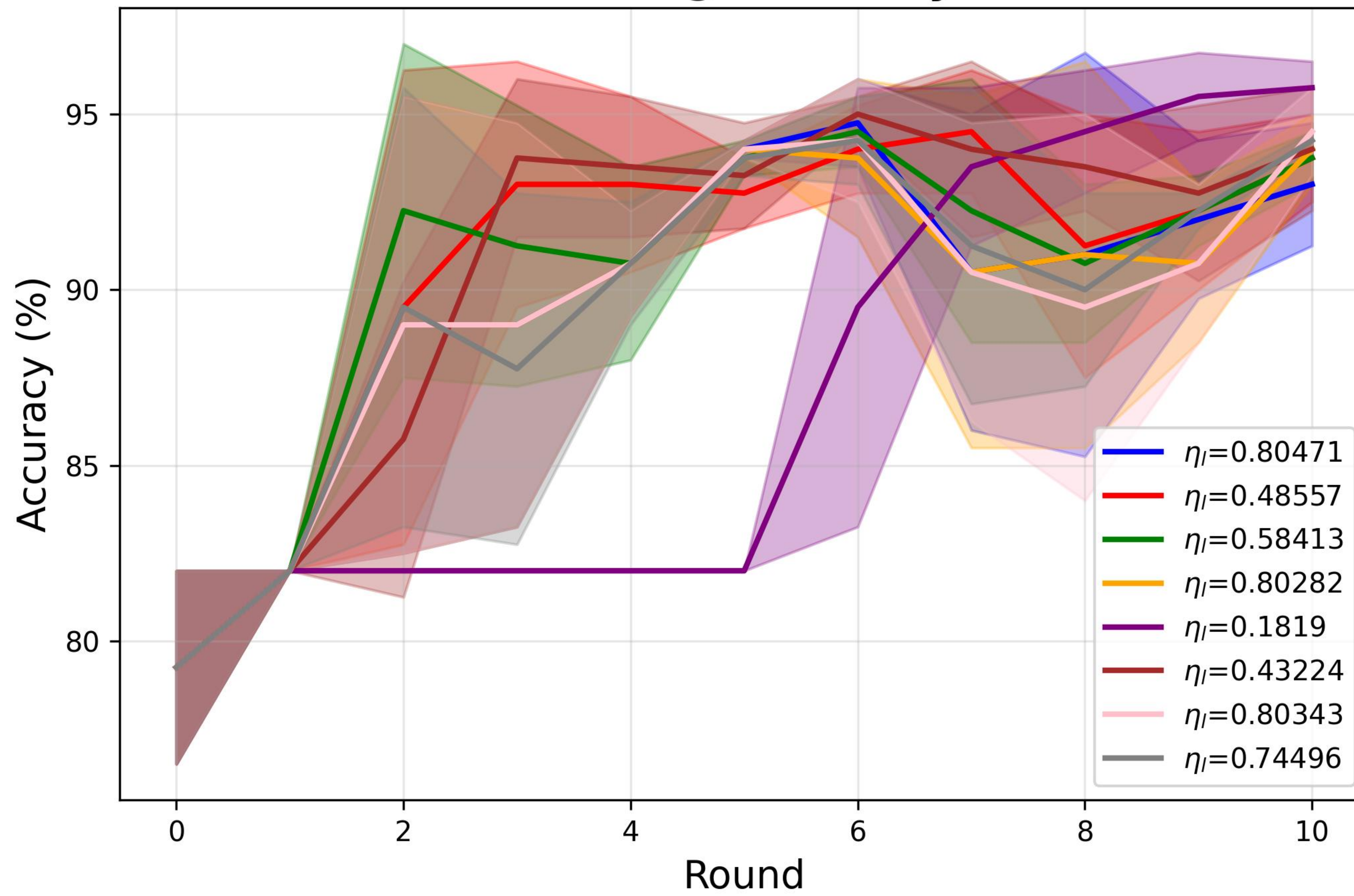
FedAvg Accuracy
