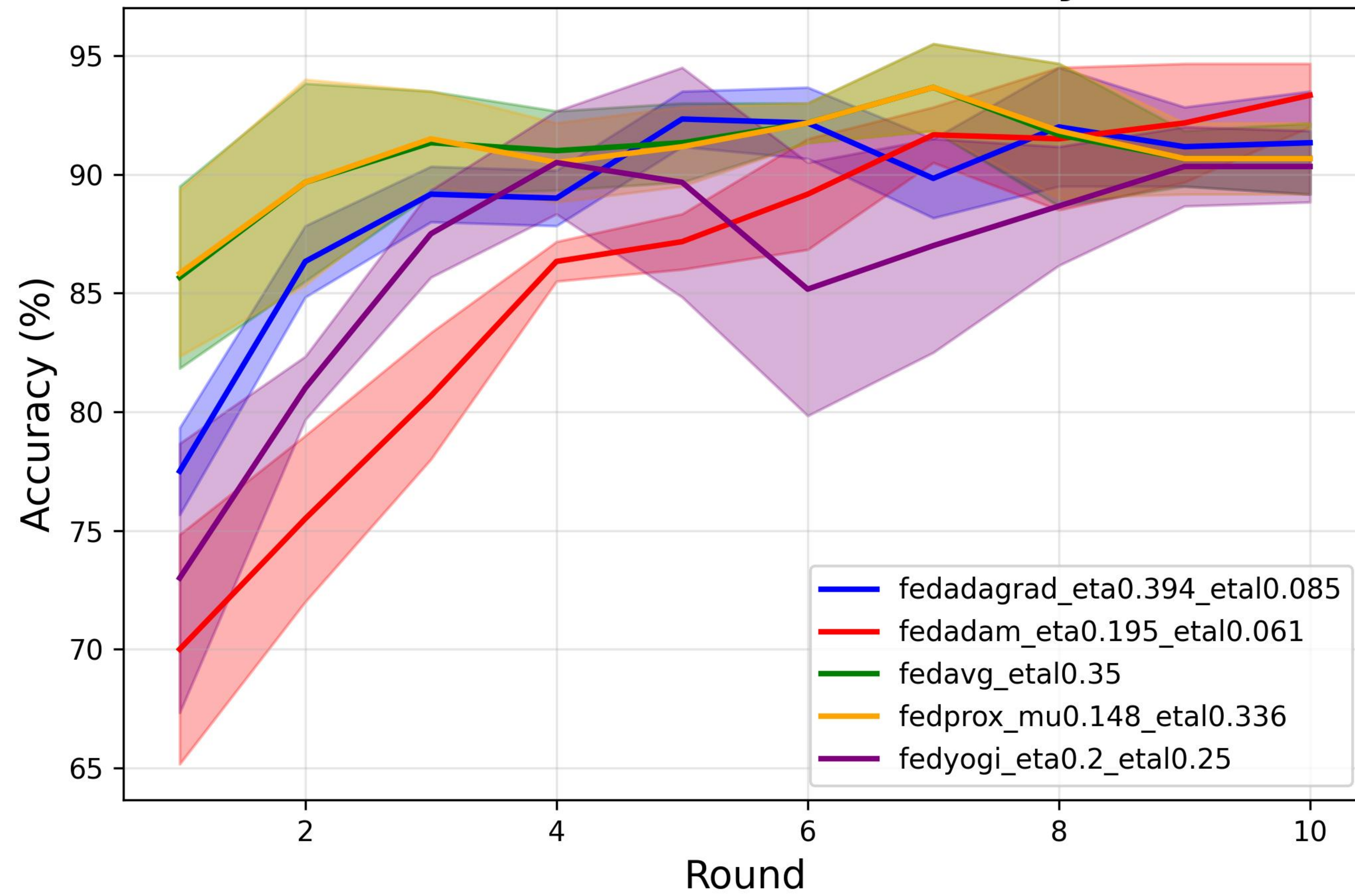
Non-IID Noiseless Accuracy
