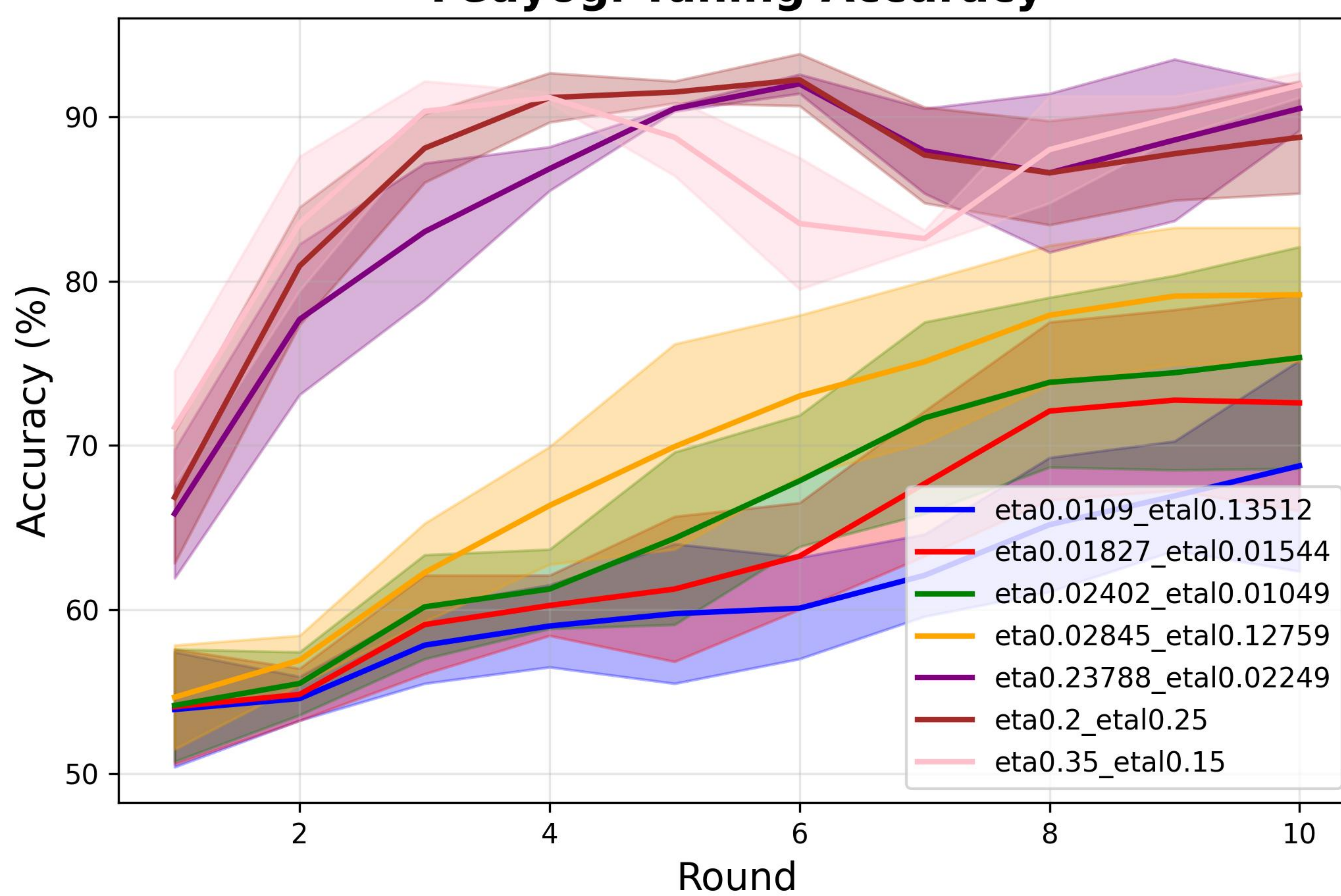
Fedyogi Tuning Accuracy
