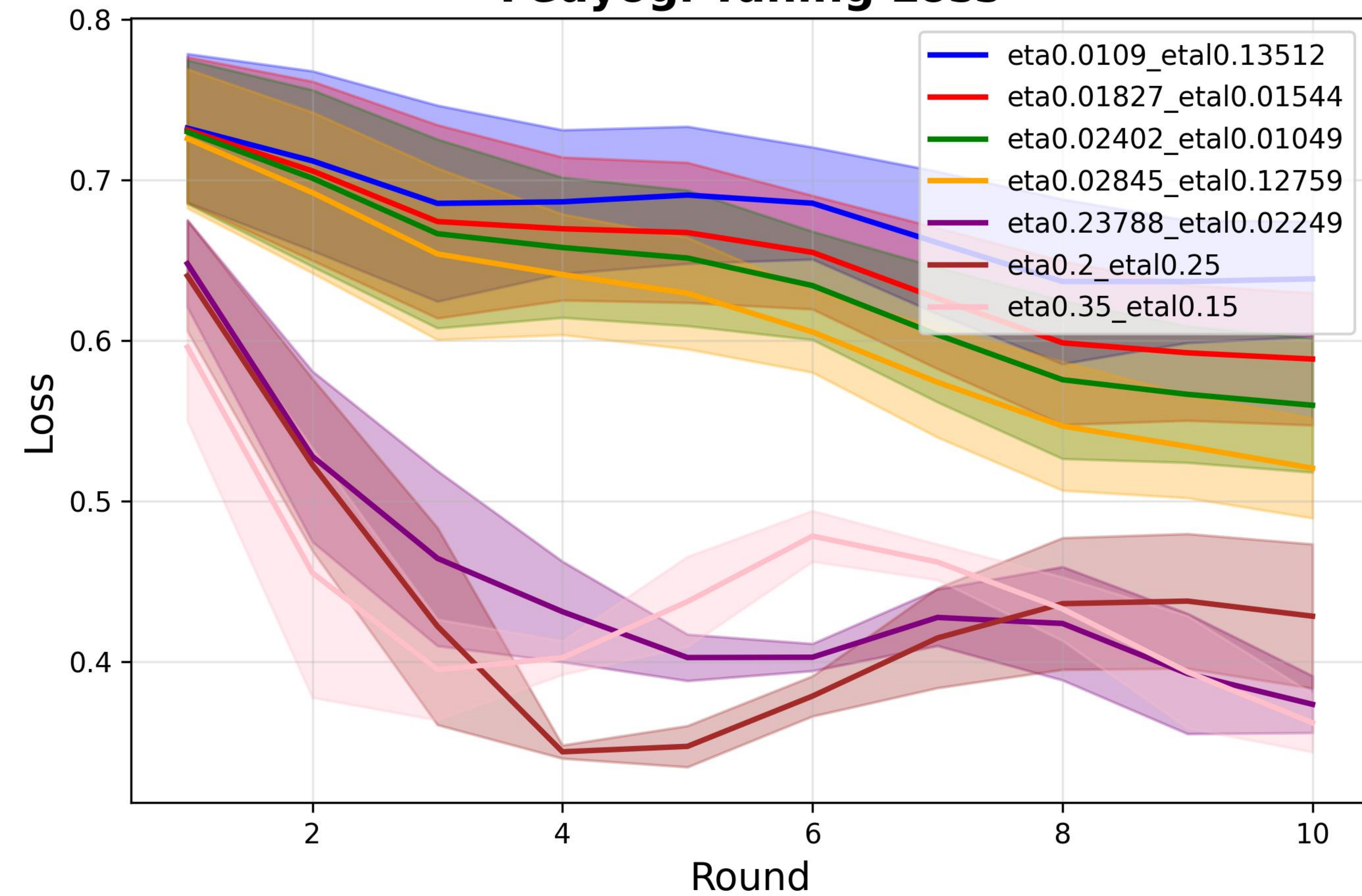
Fedyogi Tuning Loss
