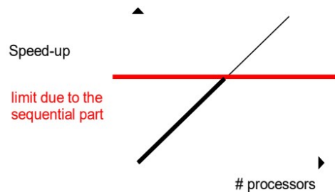
Figure 23 – Real speedup.
