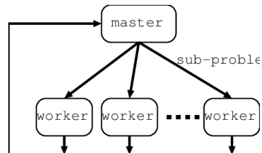
Figure 19 - Farm Pattern.
