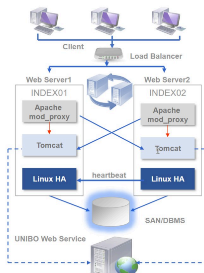
Figure 79 - ALMA architecture.
