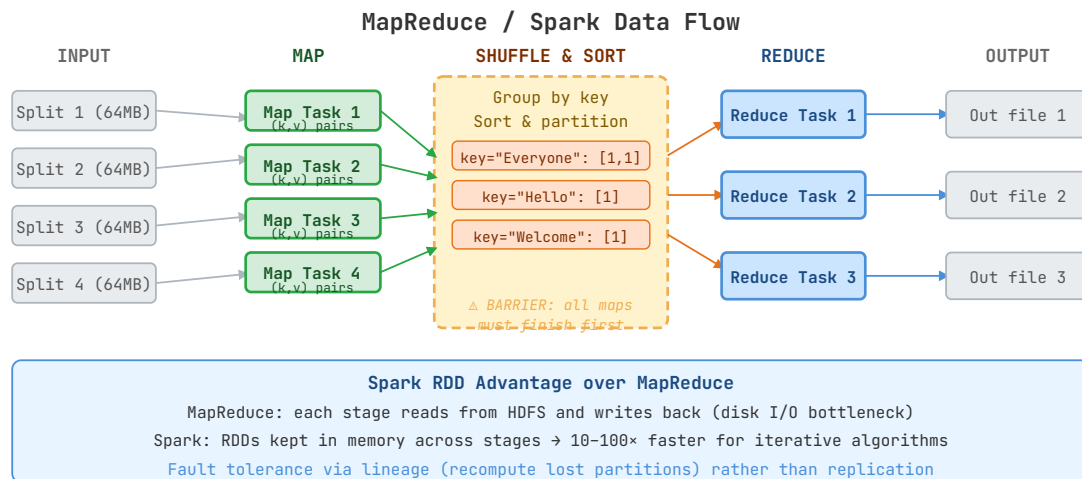
Figure 84 – MapReduce data flow: input splits → parallel Map tasks → Shuffle & Sort (global barrier) → parallel Reduce tasks → output. Spark avoids the disk I/O bottleneck by keeping RDDs in memory across stages.
