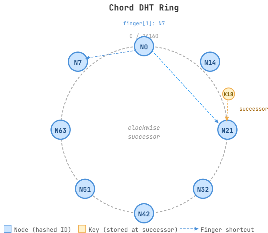
Figure 82 – Chord DHT ring: nodes placed on a 160-bit ID circle; each key is stored at its clockwise successor. Finger table shortcuts give O(\log N) lookup.
