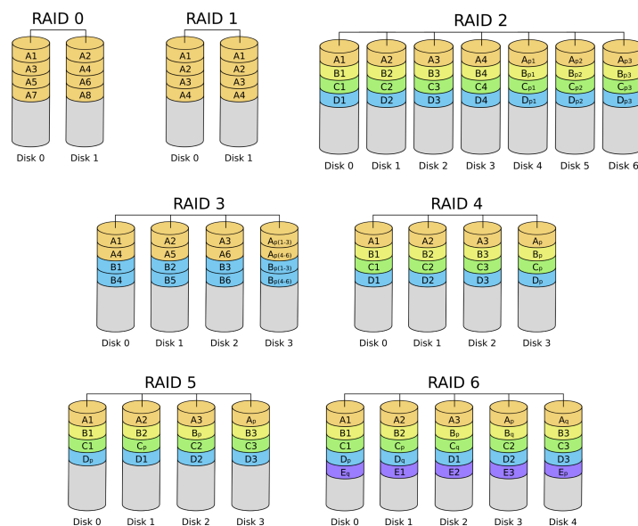
Figure 77 - RAIDs comparison.
