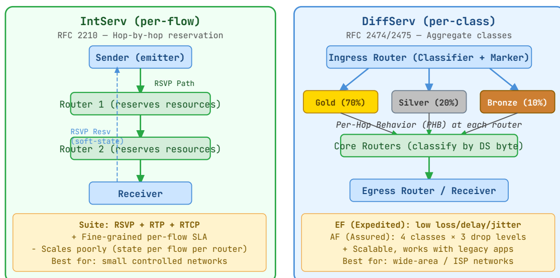
Figure 81 – IntServ (per-flow RSVP reservation, hop-by-hop) vs DiffServ (aggregate class queues, DS byte marking): the two main QoS models in IP networks.
