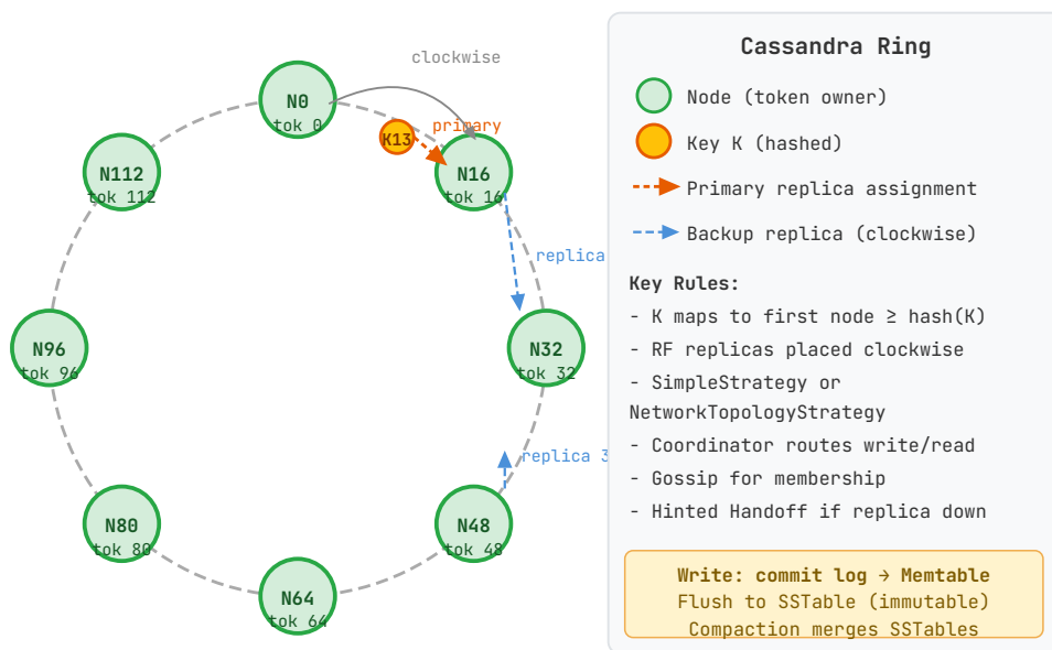
Figure 83 – Cassandra ring: nodes own token ranges; a key is routed to the first node clockwise whose token \geq \text{hash}(\text{key}) . Replicas follow clockwise. Writes go to commit log then Memtable, flushed as immutable SSTables.
