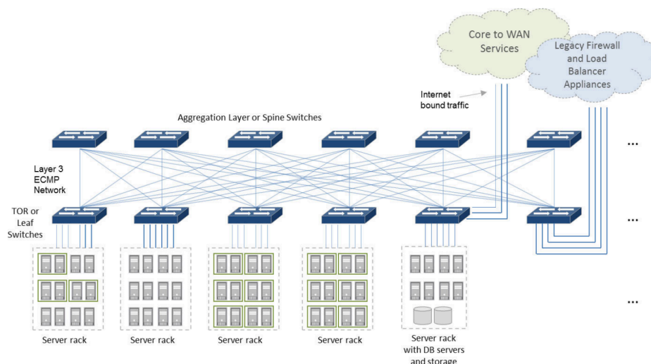
Figure 31 - Fat tree scheme.
