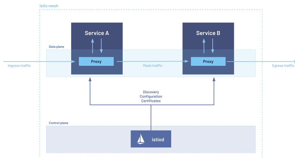
Figure 52 - Istio service mesh: Envoy sidecars in the data plane, Istiod in the control plane.
