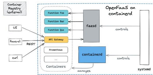
Figure 71 - faasd scheme.
