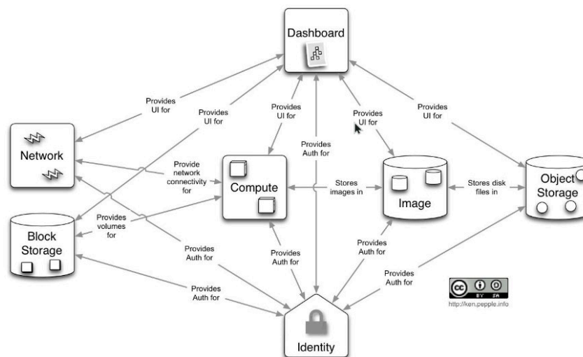
Figure 54 - Openstack.
