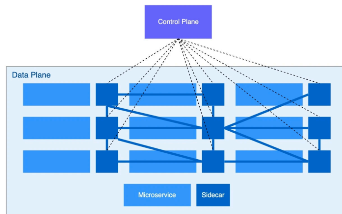
Figure 51 - Service mesh.
