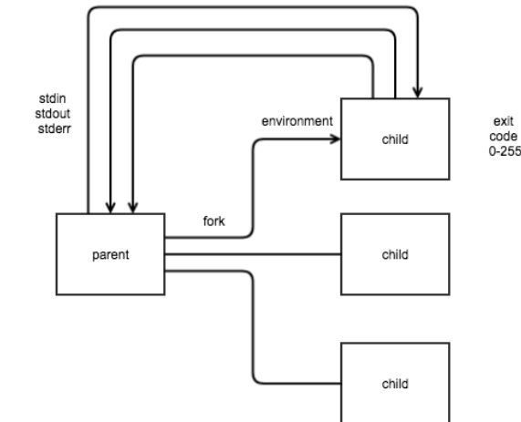
Figure 69 - Watchdog forking.
