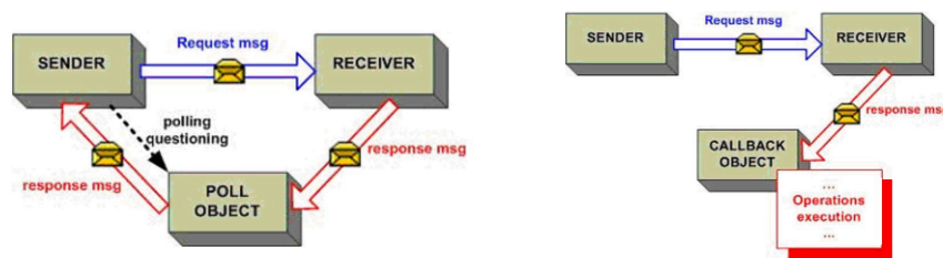
Figure 36 - Poll object (left) vs. Callback object (right).
