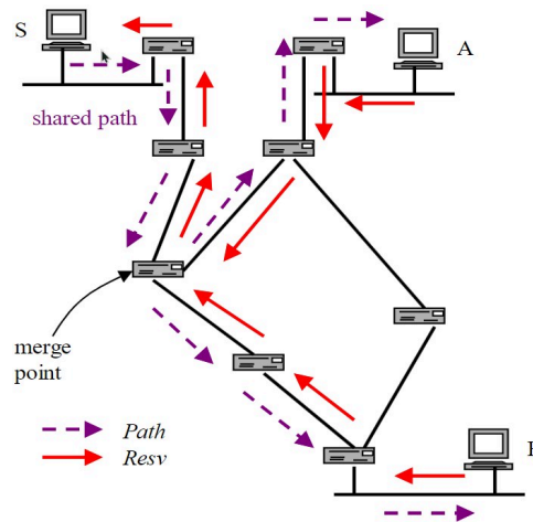
Figure 84 - RSVP Path and Resv flow.
