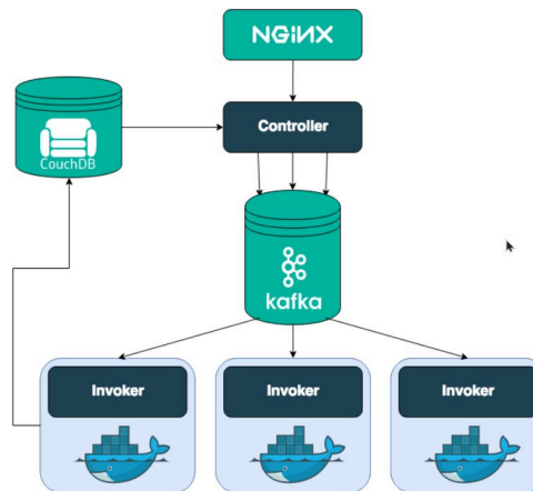
Figure 72 – OpenWhisk architecture.
