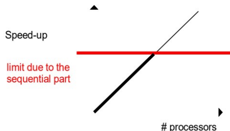
Figure 23 – Real speedup.
