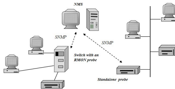
Figure 90 - RMON probe.
