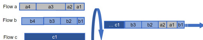
Figure 92 – Fair queuing example.
