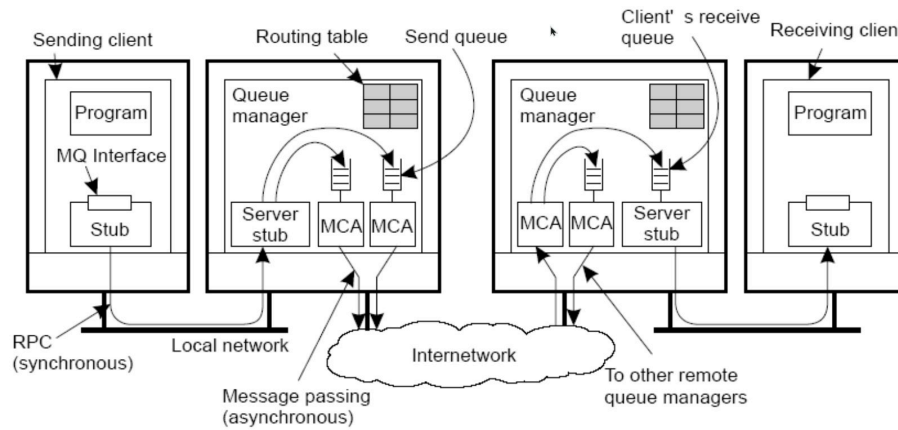
Figure 39 - MQSeries MOM IBM scheme.
