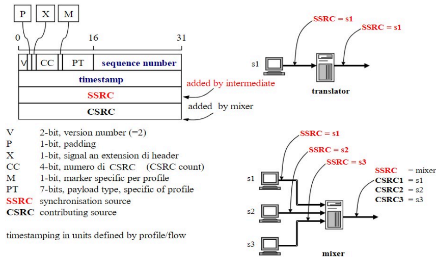
Figure 85 - RTP packet and flow scheme.
