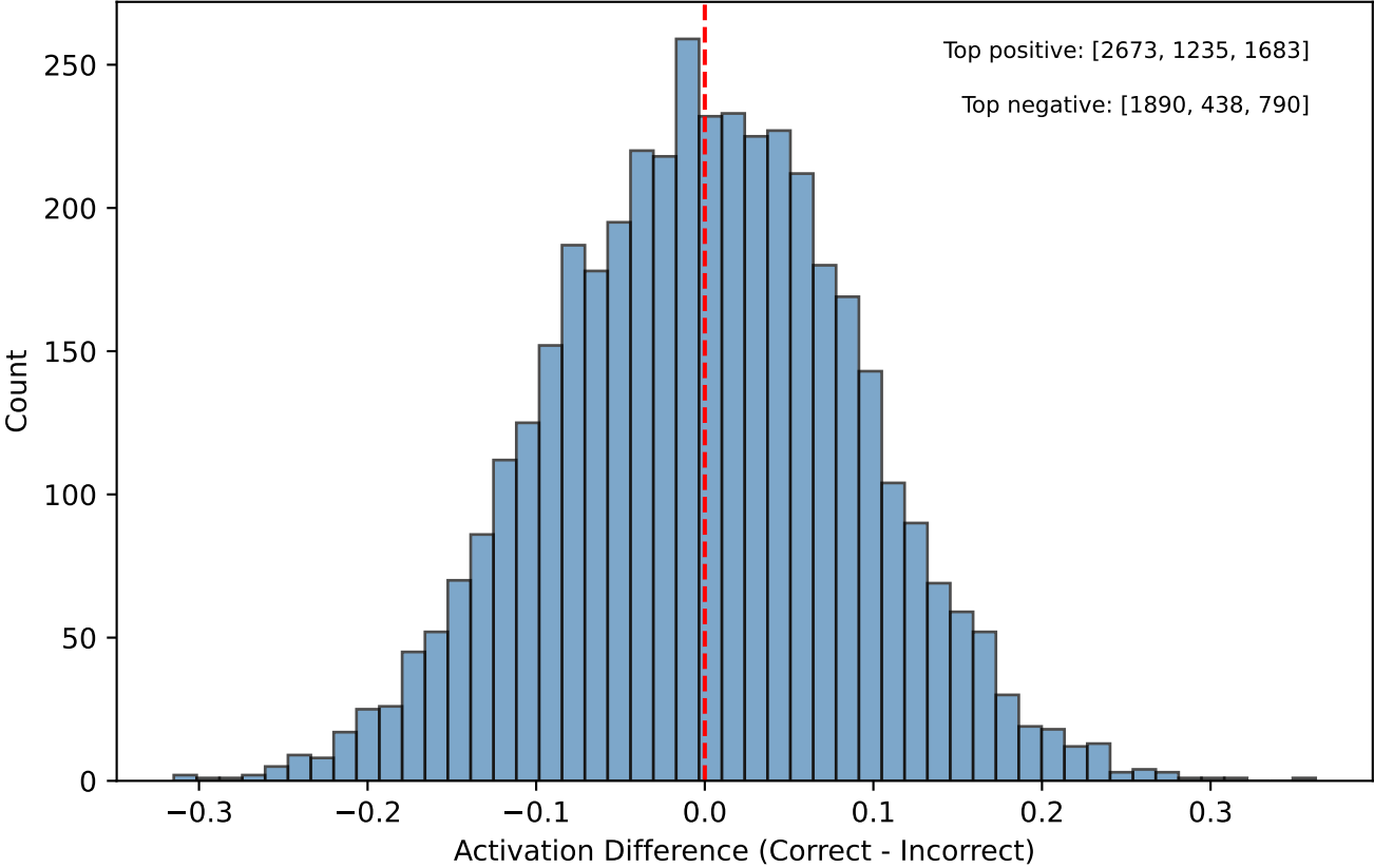
Layer 21: Neuron Activation Differences
