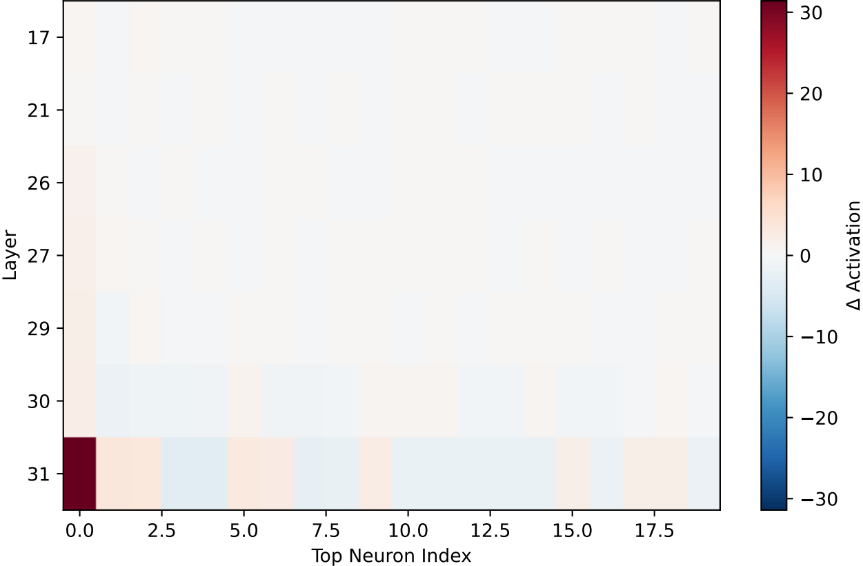
Top Neurons by Activation Difference
