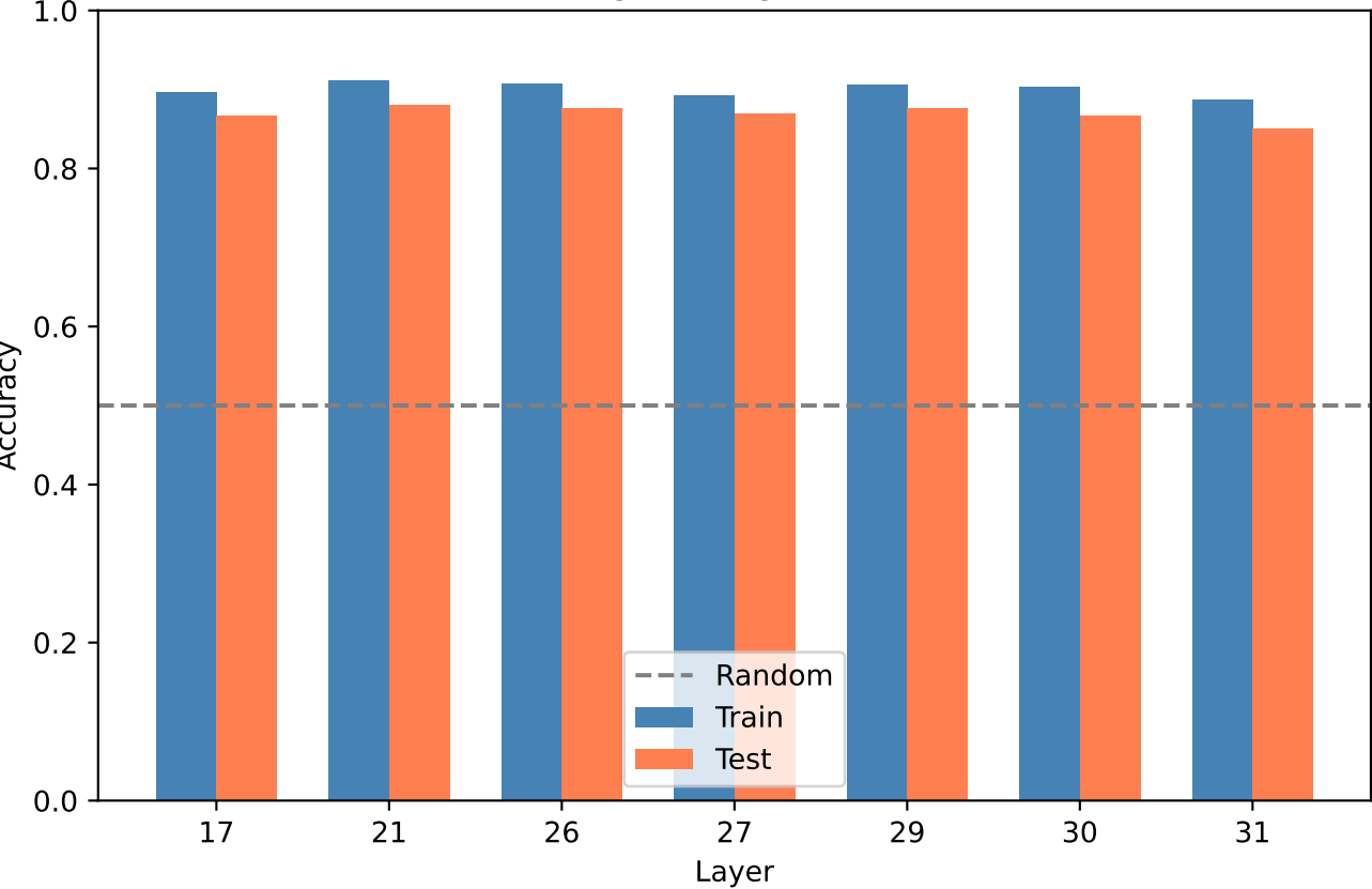
Neuron Activations → Correctness (Logistic Regression)
