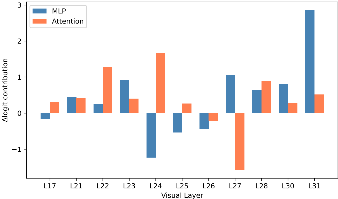
MLP vs Attention (Visual Layers Only)
