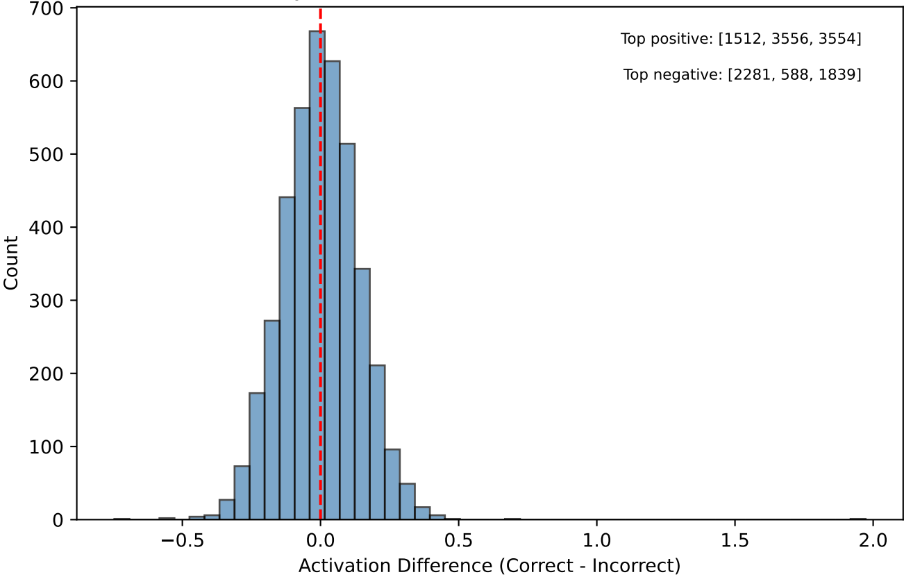
Layer 29: Neuron Activation Differences
