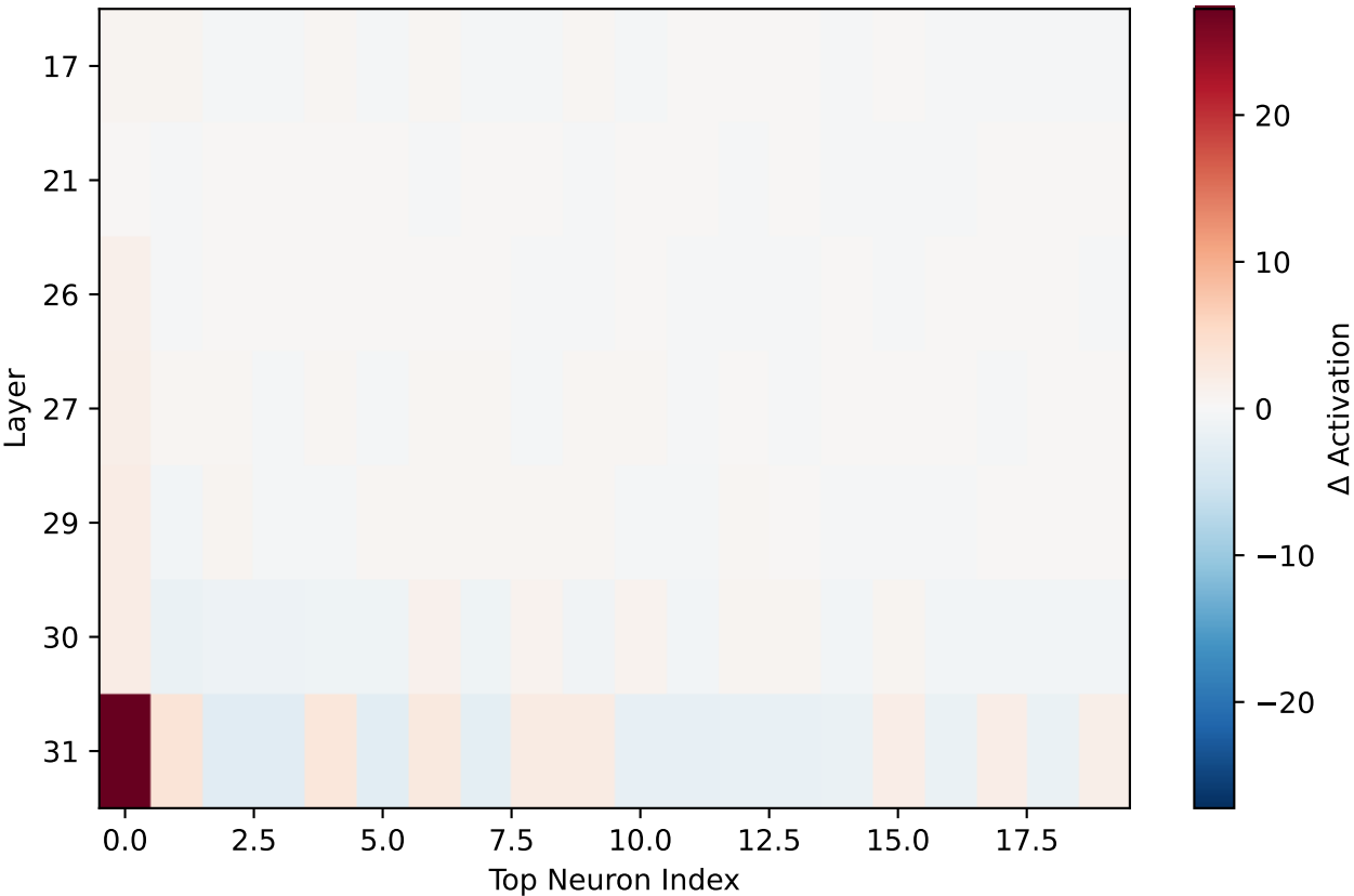
Top Neurons by Activation Difference
