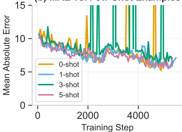
(b) MAE vs. Few-Shot Examples
