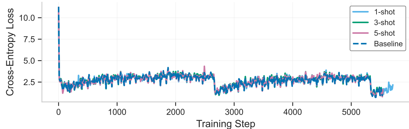
Training Cross-Entropy Loss Across Training
