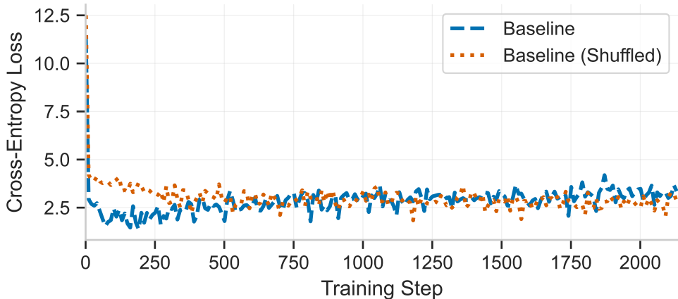
Baseline vs. Shuffled: Train Cross-Entropy
