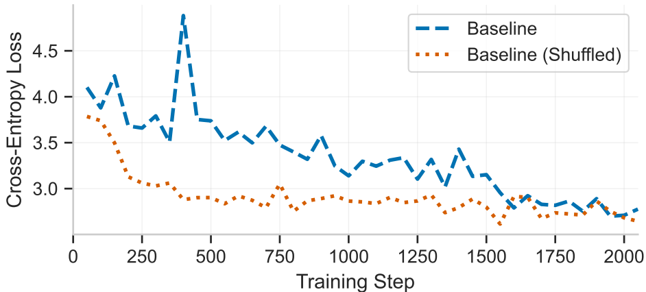
Baseline vs. Shuffled: Eval Cross-Entropy
