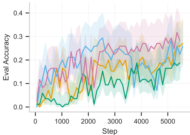
(a) Evaluation Accuracy
