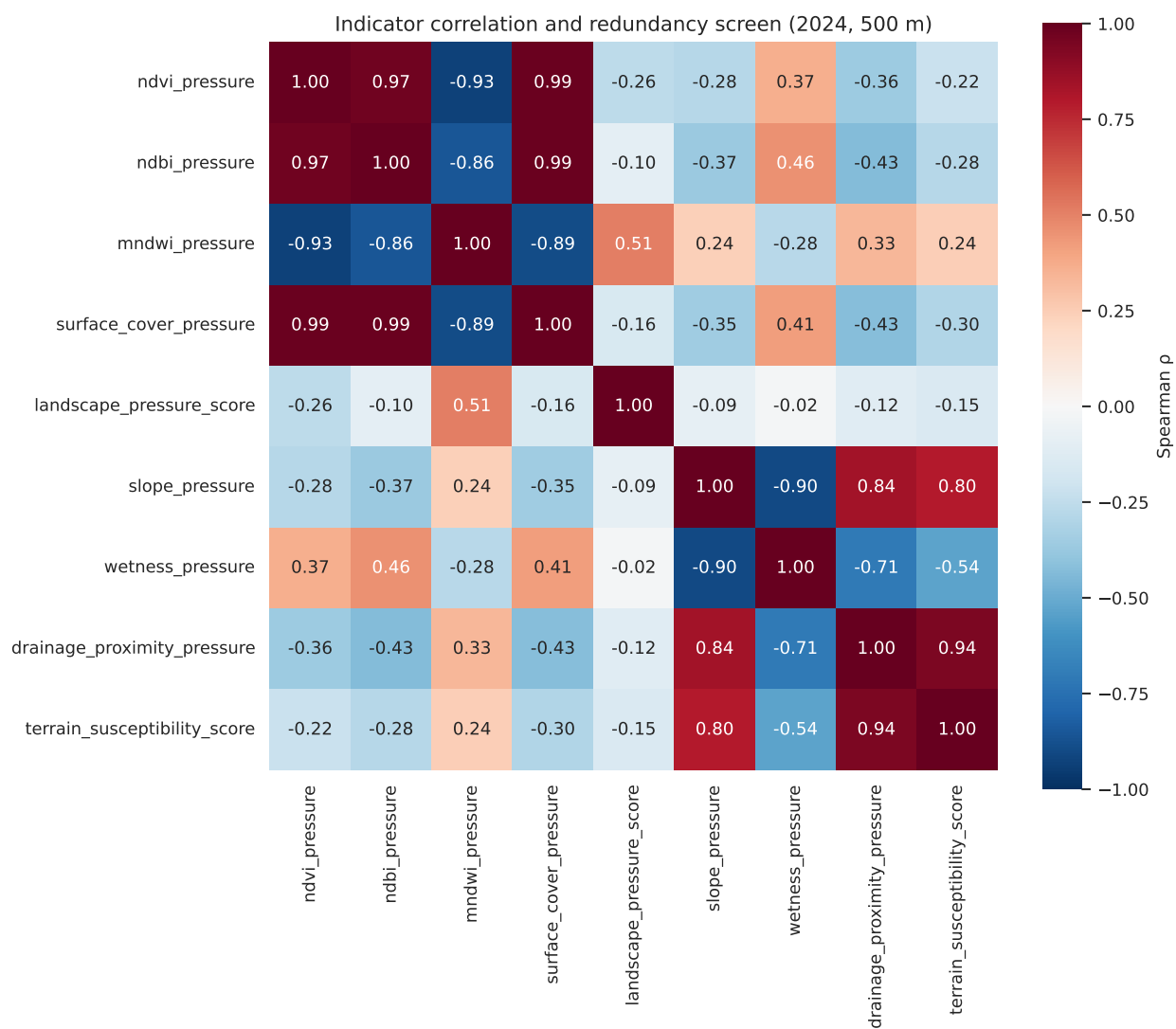
Figure S3: Dependence among component-level indicator ranks.
