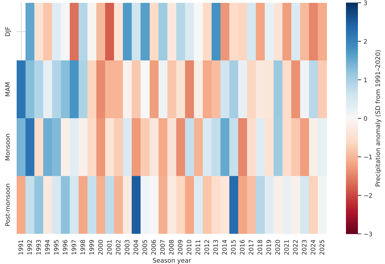
Seasonal and monsoon precipitation anomalies
