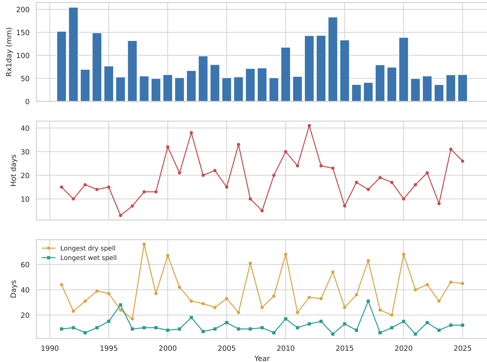
Extreme rainfall, heat and wet/dry-spell timeline
