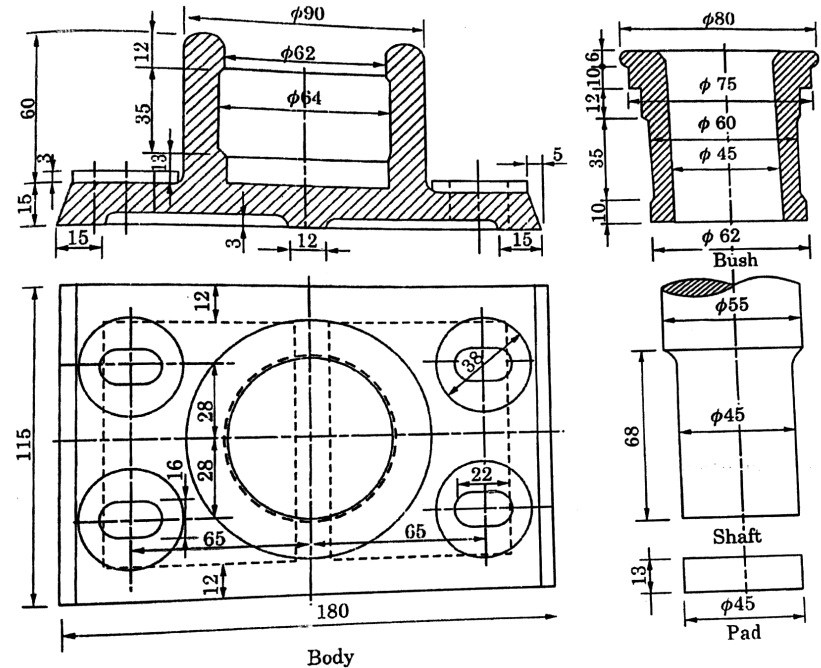
Figure1. Detail drawing of foot step bearing
