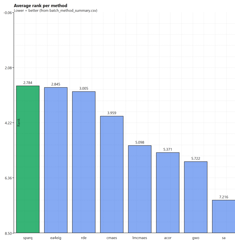
Figure 1. Average Friedman rank per optimizer across all 97 (problem, dimension) instances (lower is better), corresponding to the values in Table 2.
