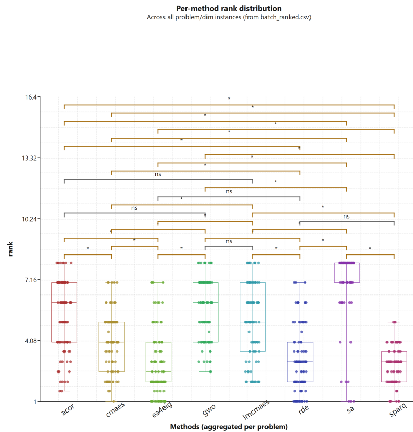
Figure 2. Per-method rank distribution across all problem instances, with pairwise Wilcoxon significance brackets. Brackets marked ns denote the five non-significant pairs listed in Table 4.
