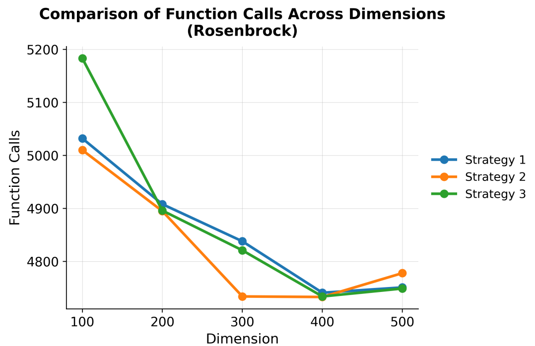
Figure 9. Comparison of objective function evaluations across problem dimensions for the three communication strategies on the Rosenbrock benchmark function.
