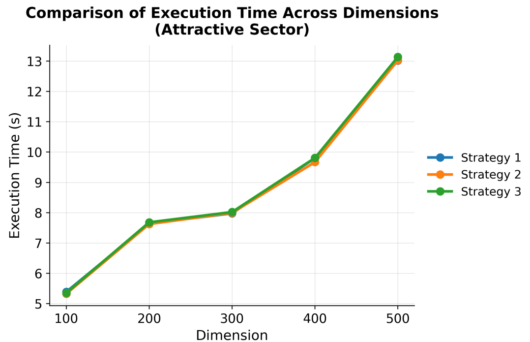
Figure 8. Comparison of execution time across problem dimensions for the three communication strategies on the Attractive Sector benchmark function.
