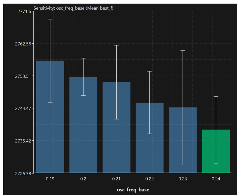
Figure 9. Mean best_f with 95% confidence intervals per value of osc_{fre\_base} on weatherirrigation ( D = 30 ). Green bar: optimal setting ( osc_{fre\_base} = 0.24 )
