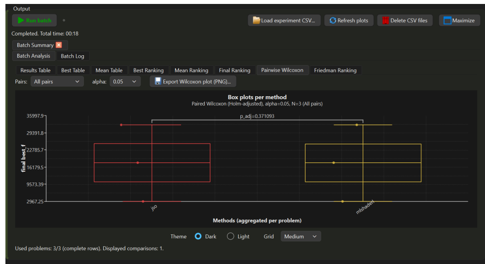
Figure 5. Pairwise Wilcoxon box plots for jSO vs. mLSHADE-RL aggregated over three Economic Load Dispatch problems (N = 3), with Holm-adjusted p-value ( p_{adj} = 0.371 , \alpha = 0.05 ), indicating no statistically significant difference between the two methods
