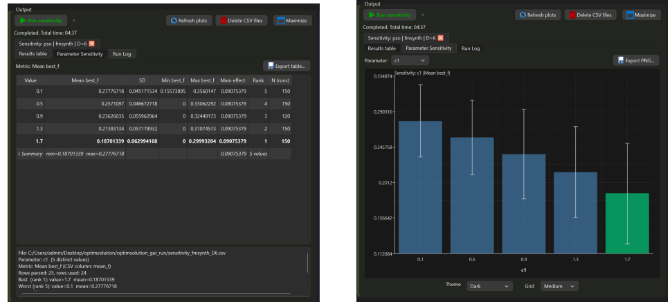
Figure 10. Method sensitivity analysis: PSO cognitive acceleration coefficient c_1 \in \{0.1, 0.5, 0.9, 1.3, 1.7\} on the FM Synthesizer Parameter Estimation problem (fmsynth, D = 6 ), 150 independent runs. Bold row: optimal setting ( c_1 = 1.7 , rank 1).
