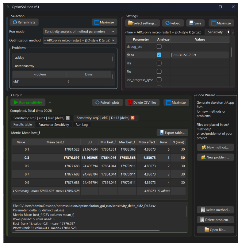
Figure 6. Method sensitivity GUI: ARQ2 parameter delta \in \{0.1, 0.3, 0.5, 0.7, 0.9\} on eld1 (D = 6) and eld2 (D = 13)
