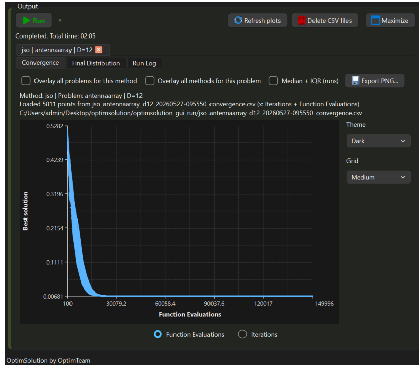
Figure 13. GUI output for the same experiment: convergence curves of the 30 independent runs and total elapsed time of 125 s (02:05), confirming identical solution quality at half the wall-clock time.
