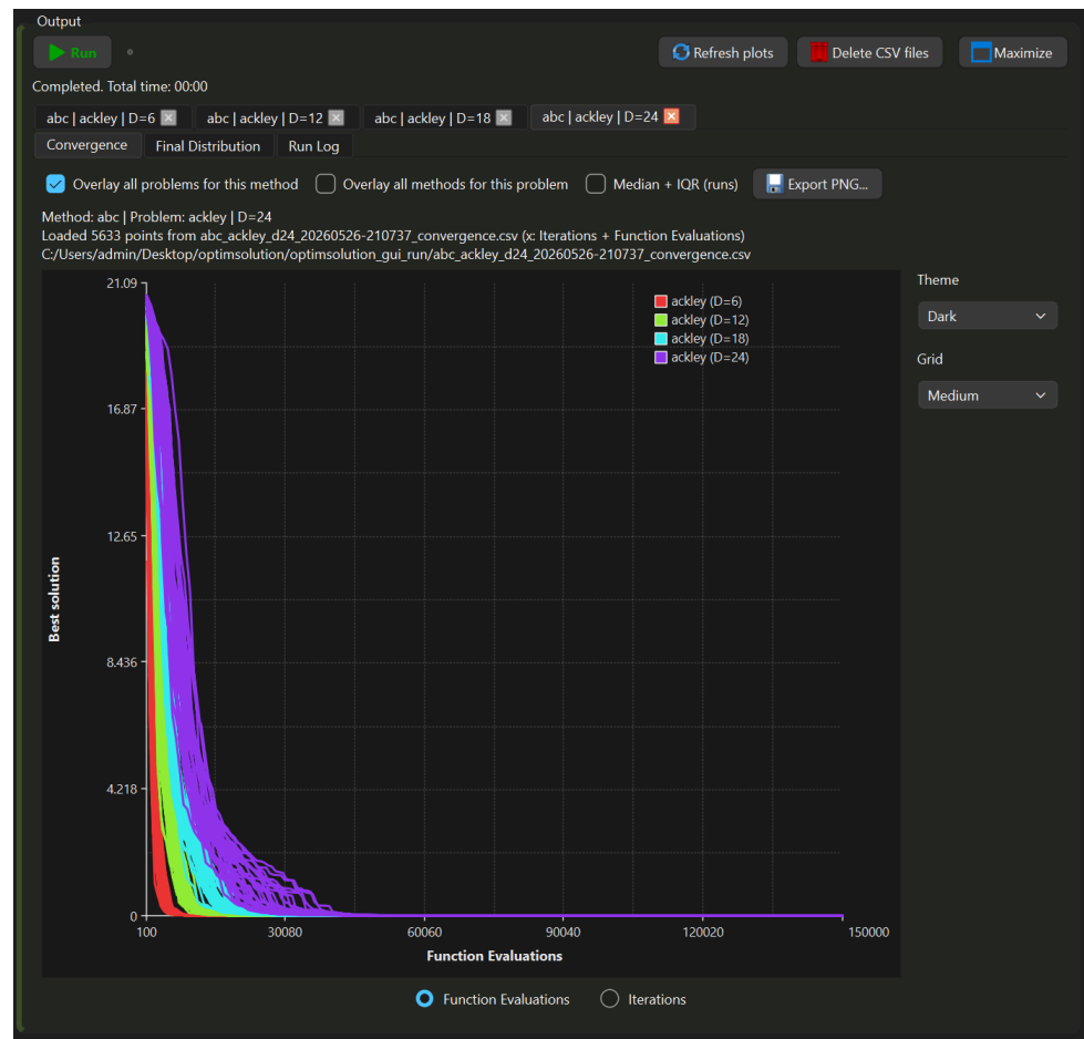
Figure 3. Convergence curves of ABC on the Ackley function for D = 6, 12, 18 , and 24 . Each colour denotes a dimensionality, same-colour lines are the 30 independent runs, reflecting method reliability and validity across problem scales
