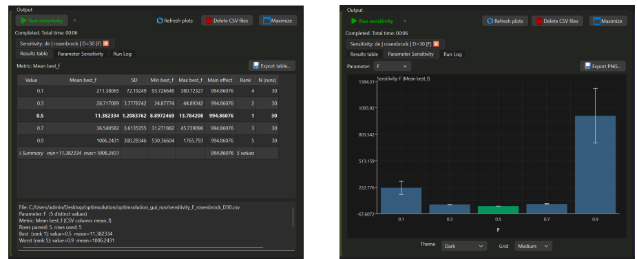
Figure 11. Method sensitivity analysis: DE scale factor F \in \{0.1, 0.3, 0.5, 0.7, 0.9\} on Rosenbrock ( D = 30 ), 30 independent runs. Bold row: optimal setting ( F = 0.5 , rank 1).
