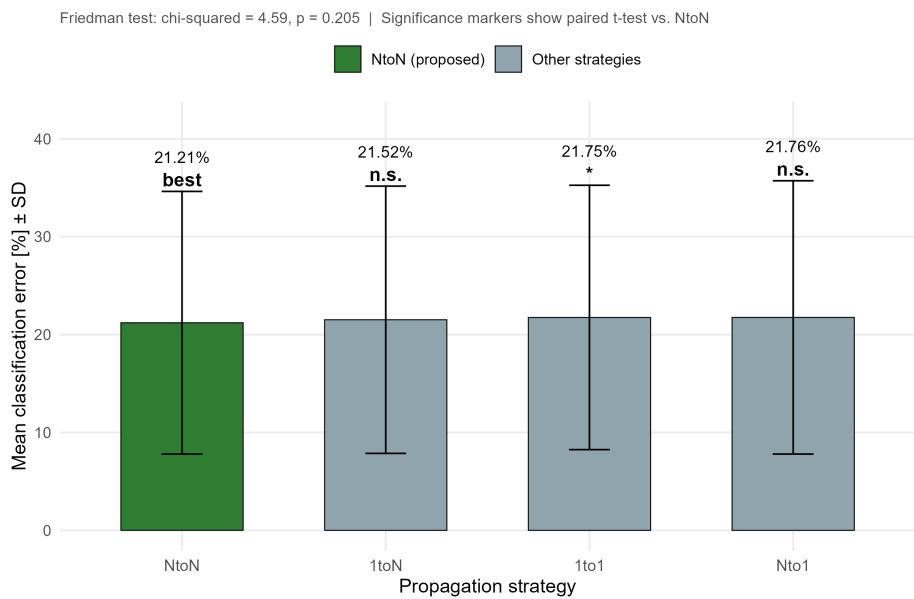
Figure 2. Mean classification error of OPSO under four solution-propagation strategies.
