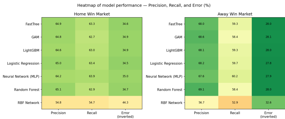
Figure 5. Heatmap of Precision, Recall and Error (%) for all seven benchmarked models on the Home Win (left) and Away Win (right) markets. The Error column is displayed inverted (100 – Error) so that green consistently denotes better performance across all three columns; the numeric labels show the original, non-inverted values.
