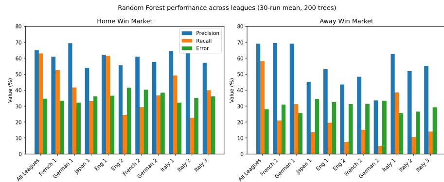
Figure 1. Mean Precision, Recall and Error (%) of the Random Forest model (200 trees, 30-run average) for the Home Win and Away Win markets, compared across the pooled dataset ("All Leagues") and the ten individually evaluated leagues.
