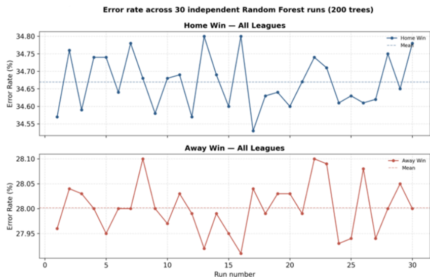
Figure 4. Error Rate (%) of the pooled ("All Leagues") Random Forest model across the 30 individual runs, for the Home Win (top) and Away Win (bottom) markets. Dashed lines mark the 30-run mean.
